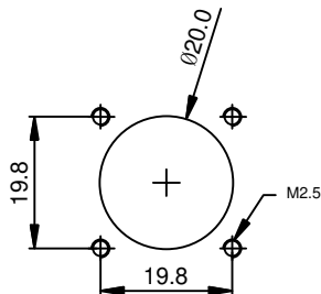
MOUNTING HOLE
