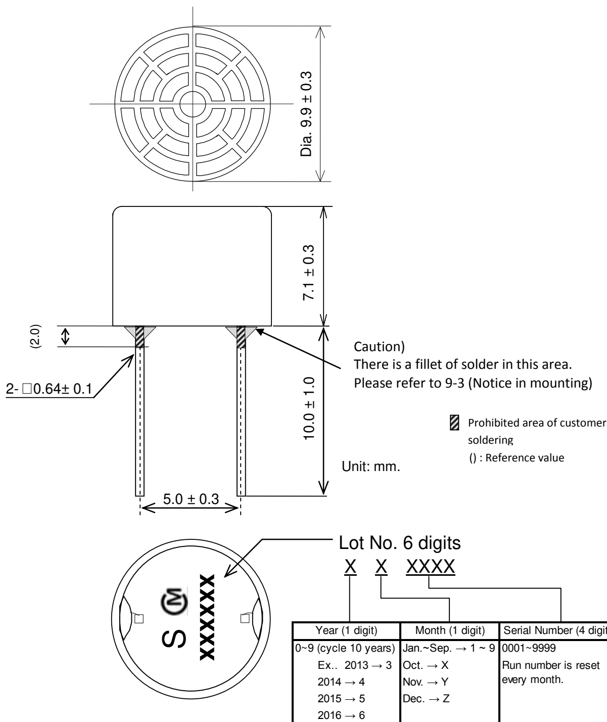
Fig.1: Product Dimension
