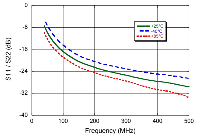
Return Loss, 100 mA Forward Bias
