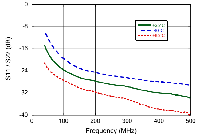
Return Loss, 20 mA Forward Bias
