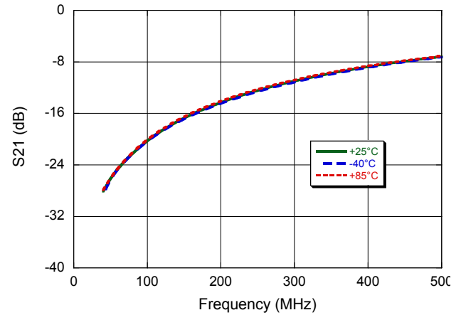
Isolation, 10 V Reverse Bias
