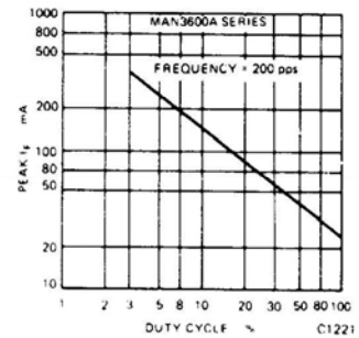
Fig. 12. Max Peak Current vs. Duty Cycle
