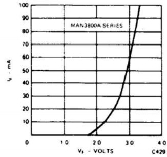
Fig. 8. Forward Current vs. Forward Voltage
