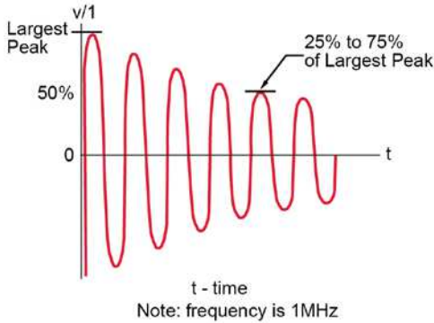
FIGURE 7 – Waveform 3
