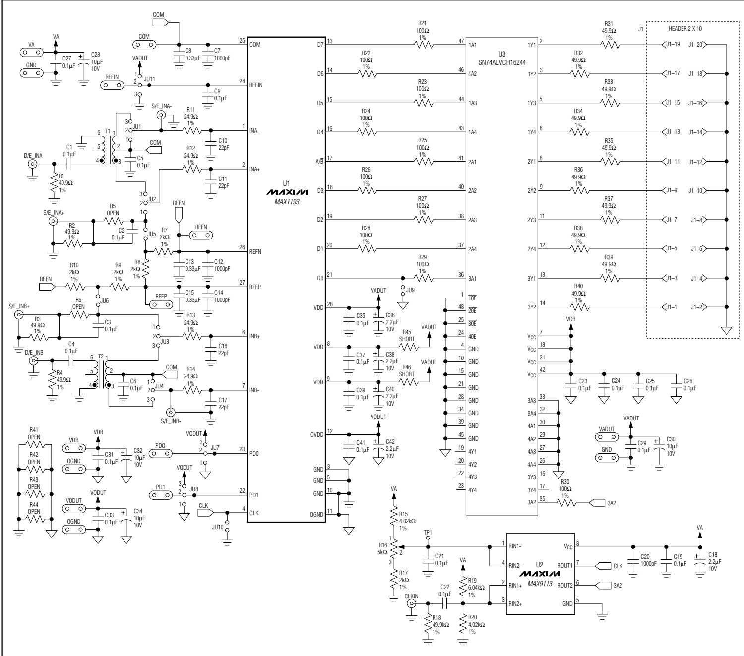
Figure 1. MAX1193 EV Kit Schematic
