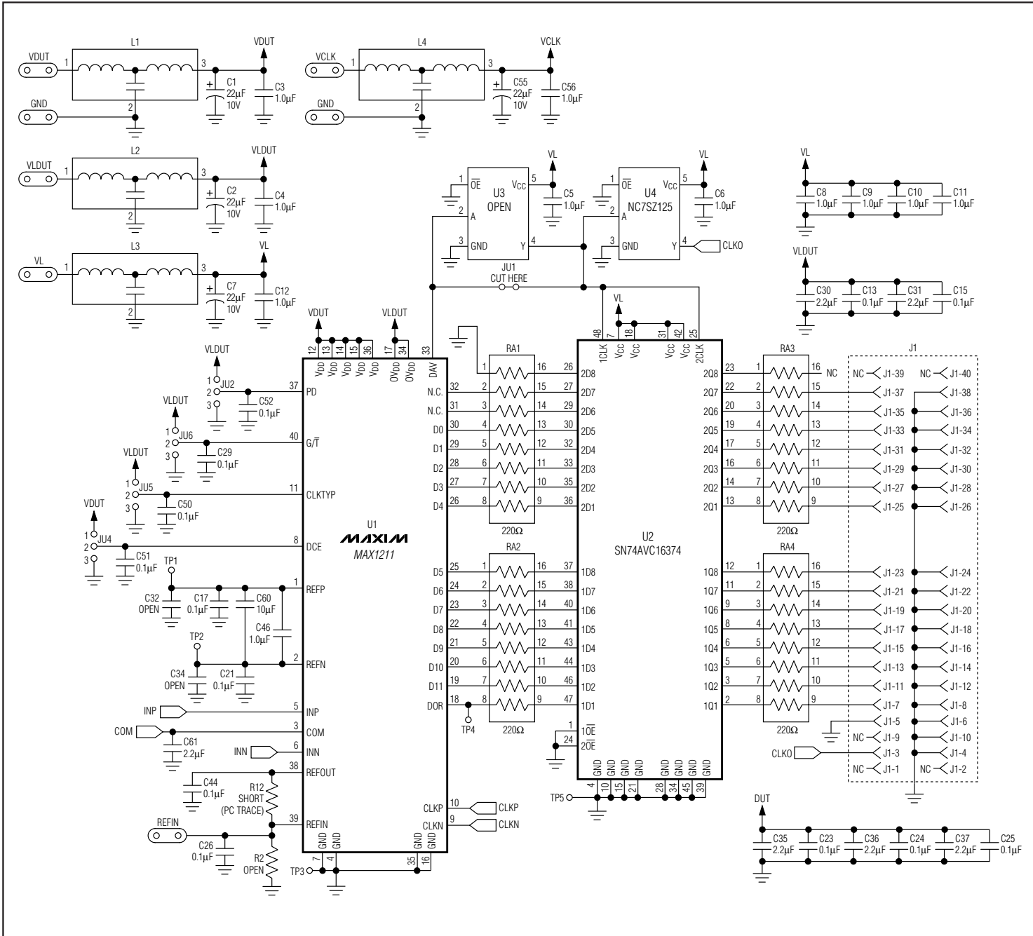
Figure 1. MAX1211 EV Kit Schematic (Sheet 1 of 2)
