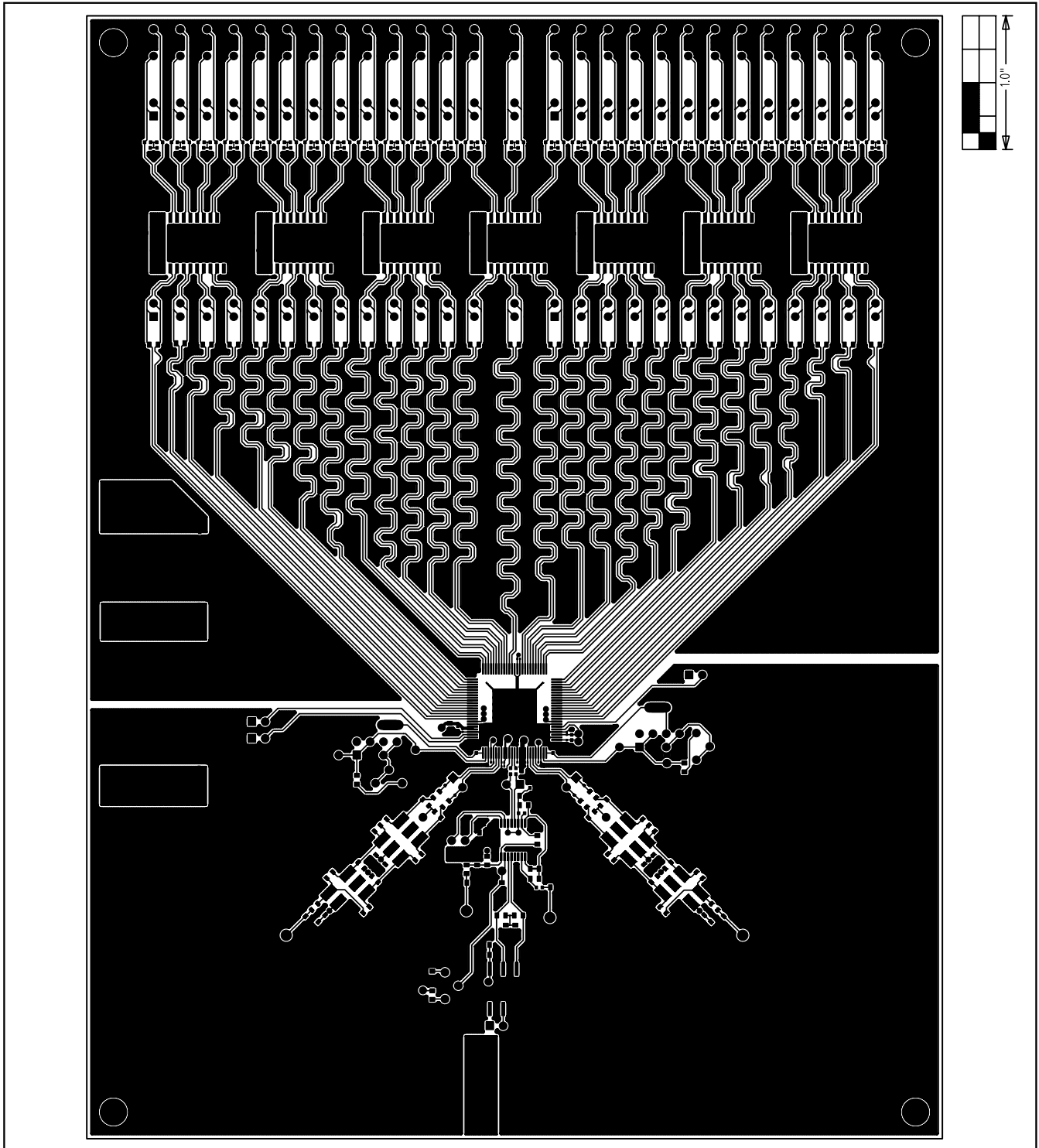
Figure 3. MAX1217/MAX1218/MAX1219 EV Kit PC Board Layout—Component Side
