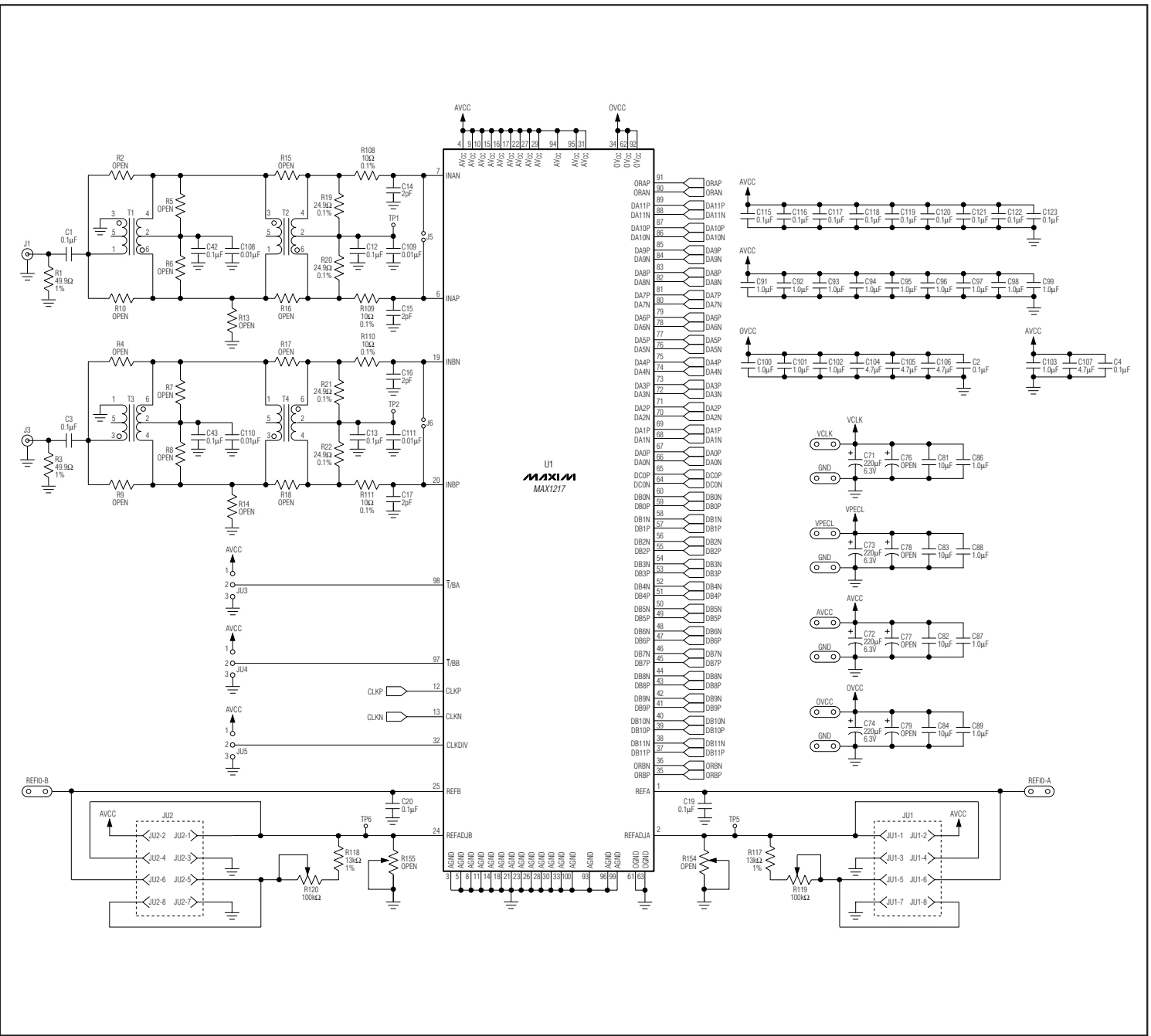
Figure 1a. MAX1217 EV Kit Schematic (Sheet 1 of 7)
