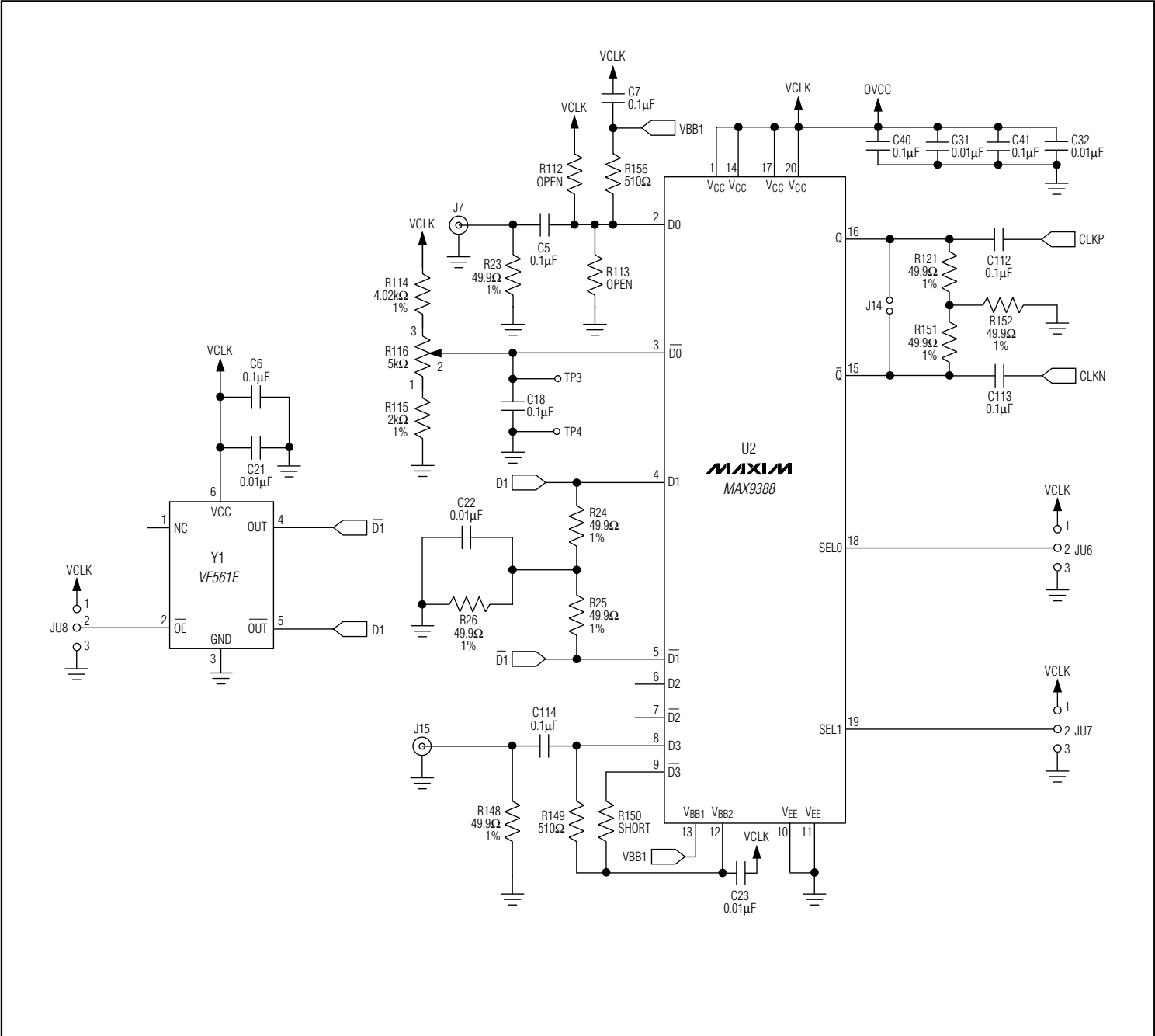
Figure 1d. MAX1217/MAX1218/MAX1219 EV Kit Schematic (Sheet 2 of 7)
