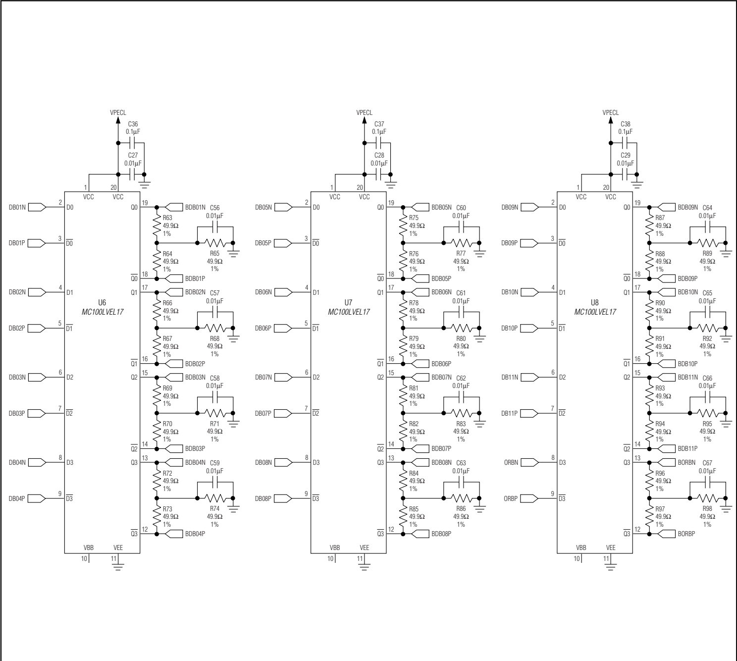
Figure 1h. MAX1217/MAX1218/MAX1219 EV Kit Schematic (Sheet 6 of 7)
