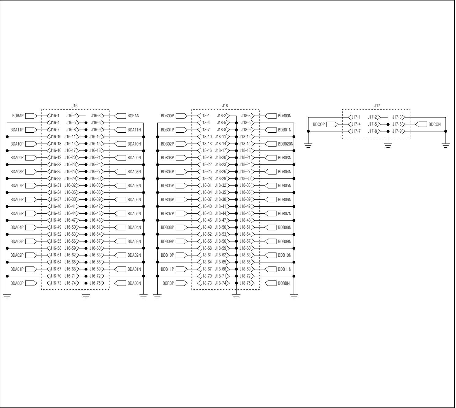
Figure 1f. MAX1217/MAX1218/MAX1219 EV Kit Schematic (Sheet 4 of 7)
