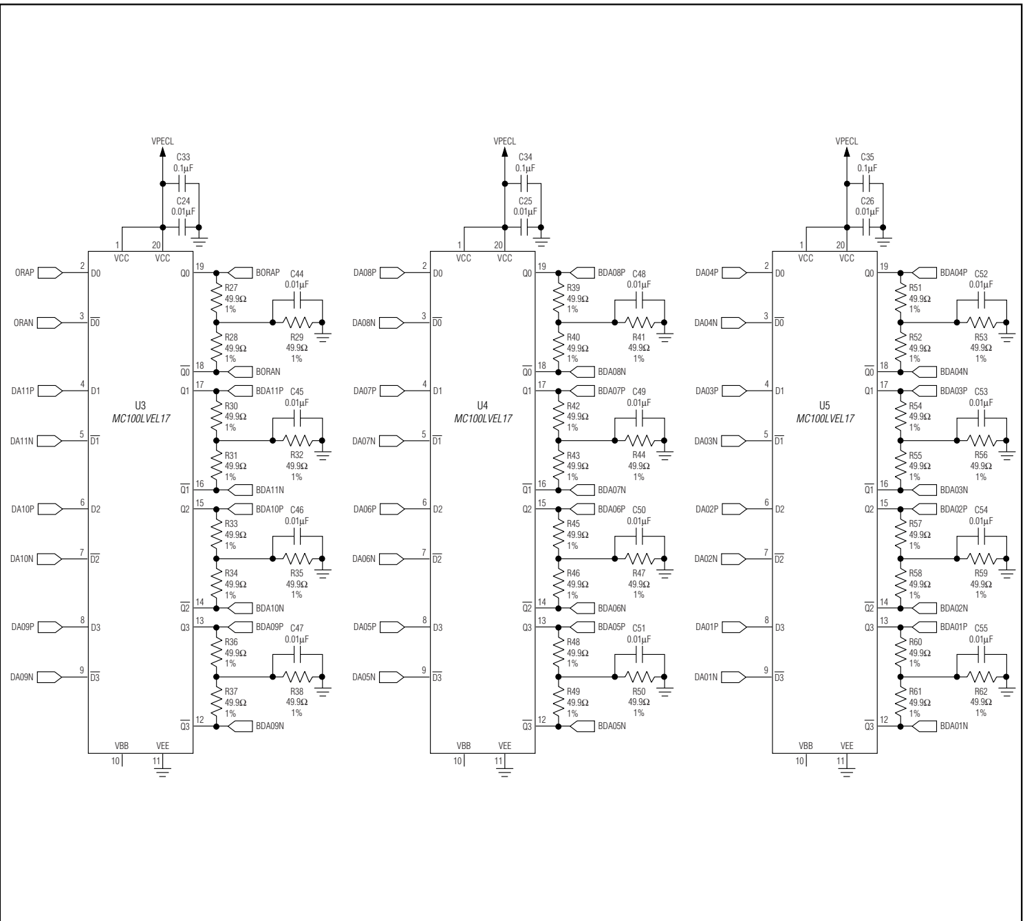
Figure 1g. MAX1217/MAX1218/MAX1219 EV Kit Schematic (Sheet 5 of 7)
