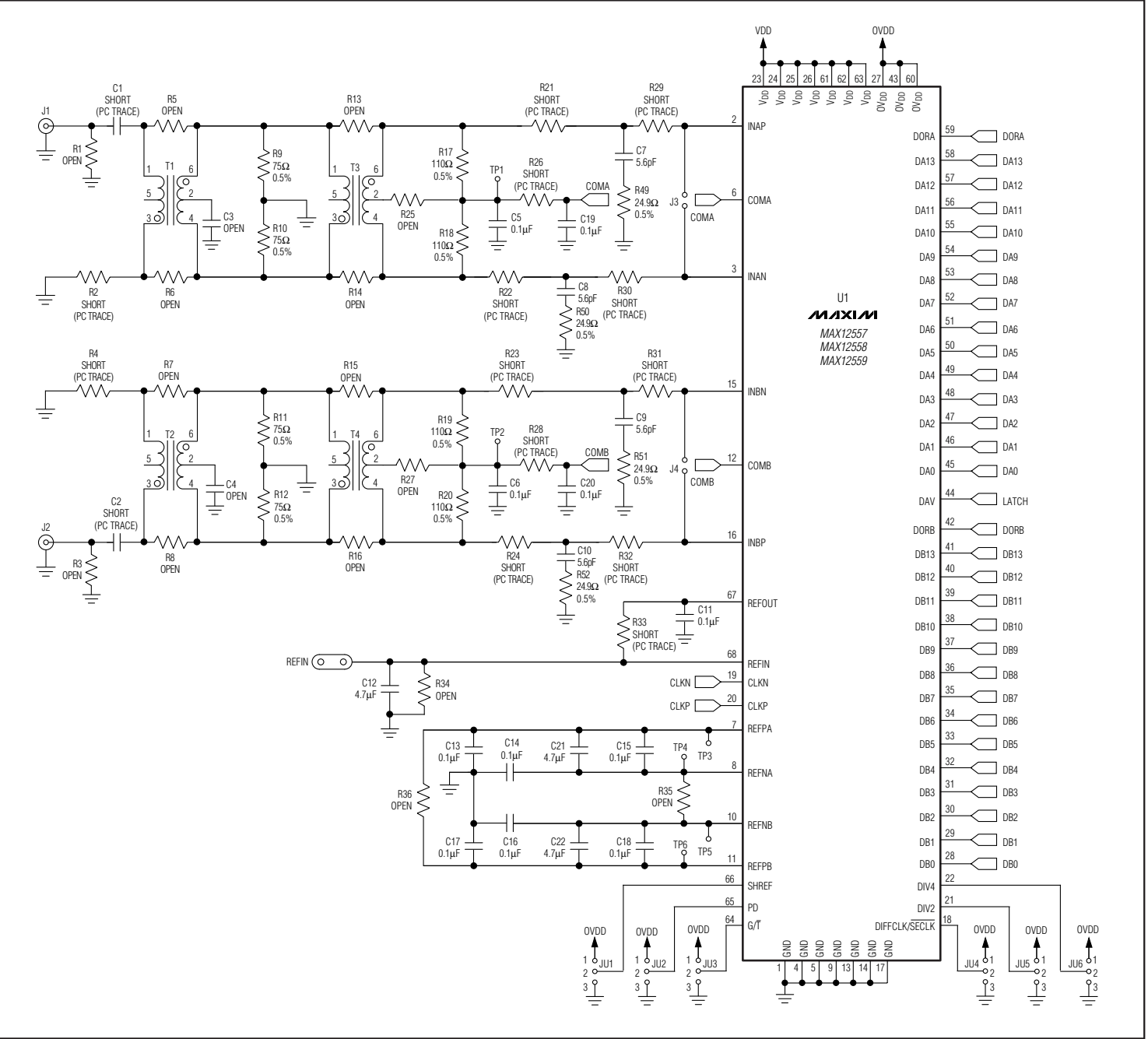
Figure 1. MAX12557/MAX12558/MAX12559 EV Kit Schematic (Sheet 1 of 4)
