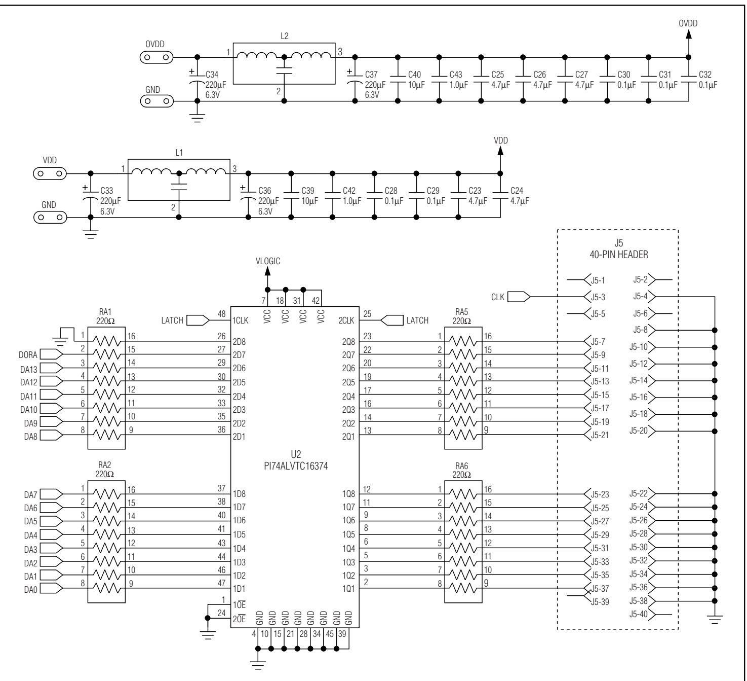
Figure 2. MAX12557/MAX12558/MAX12559 EV Kit Schematic (Sheet 2 of 4)
