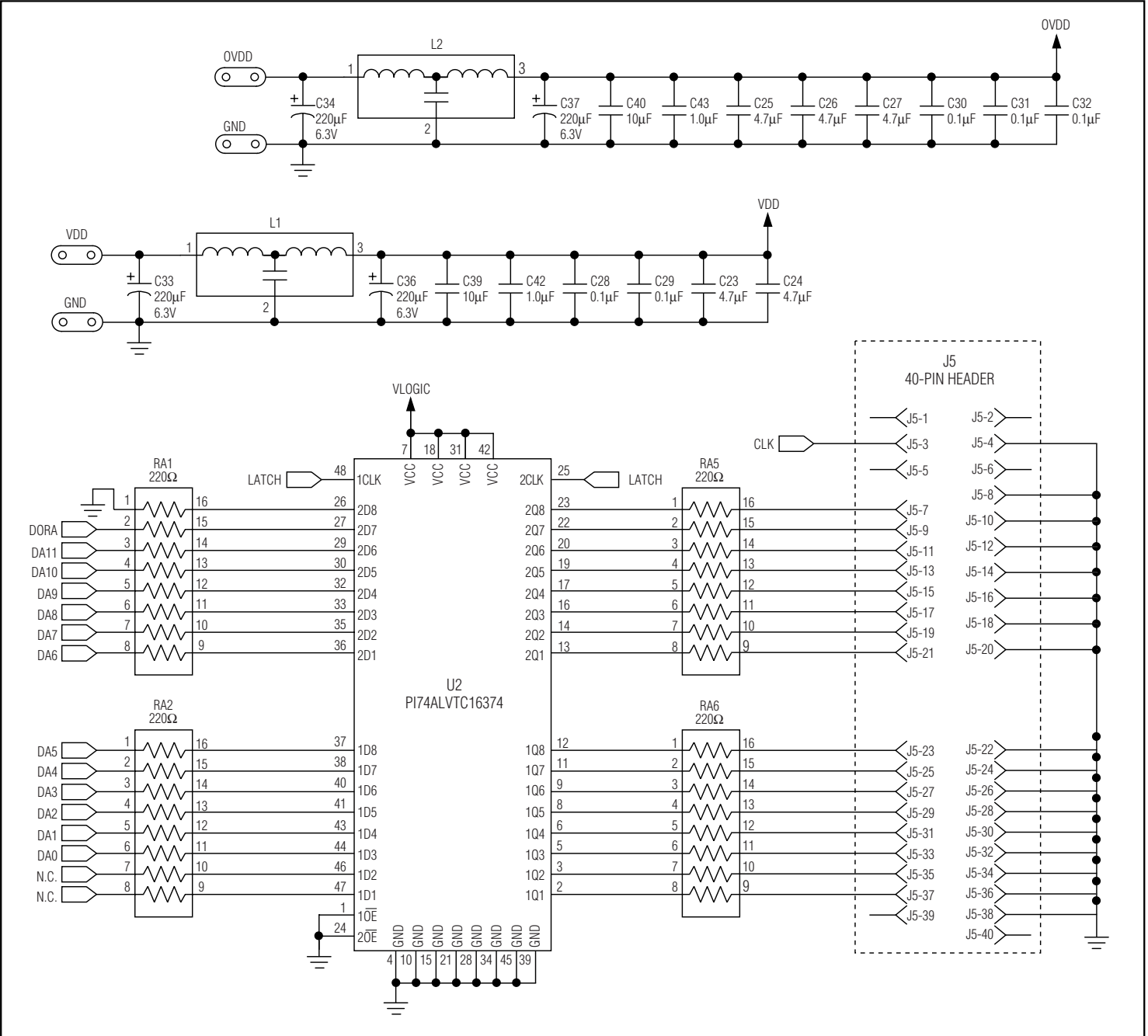
Figure 5. MAX12527/MAX12528/MAX12529 EV Kit Schematic (Sheet 2 of 4)
