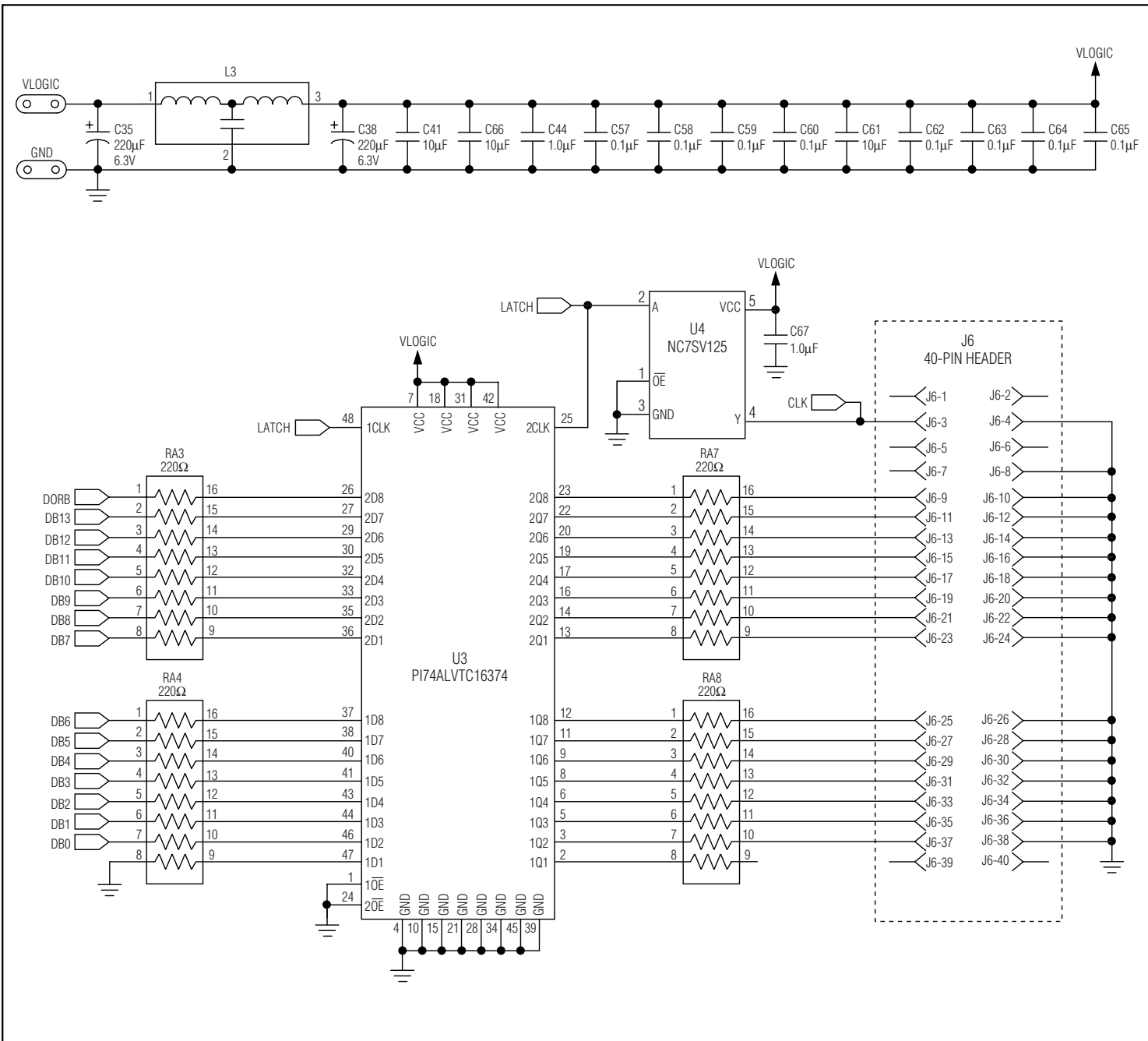
Figure 3. MAX12527/MAX12557/MAX12558/MAX12559 EV Kit Schematic (Sheet 3 of 4)
