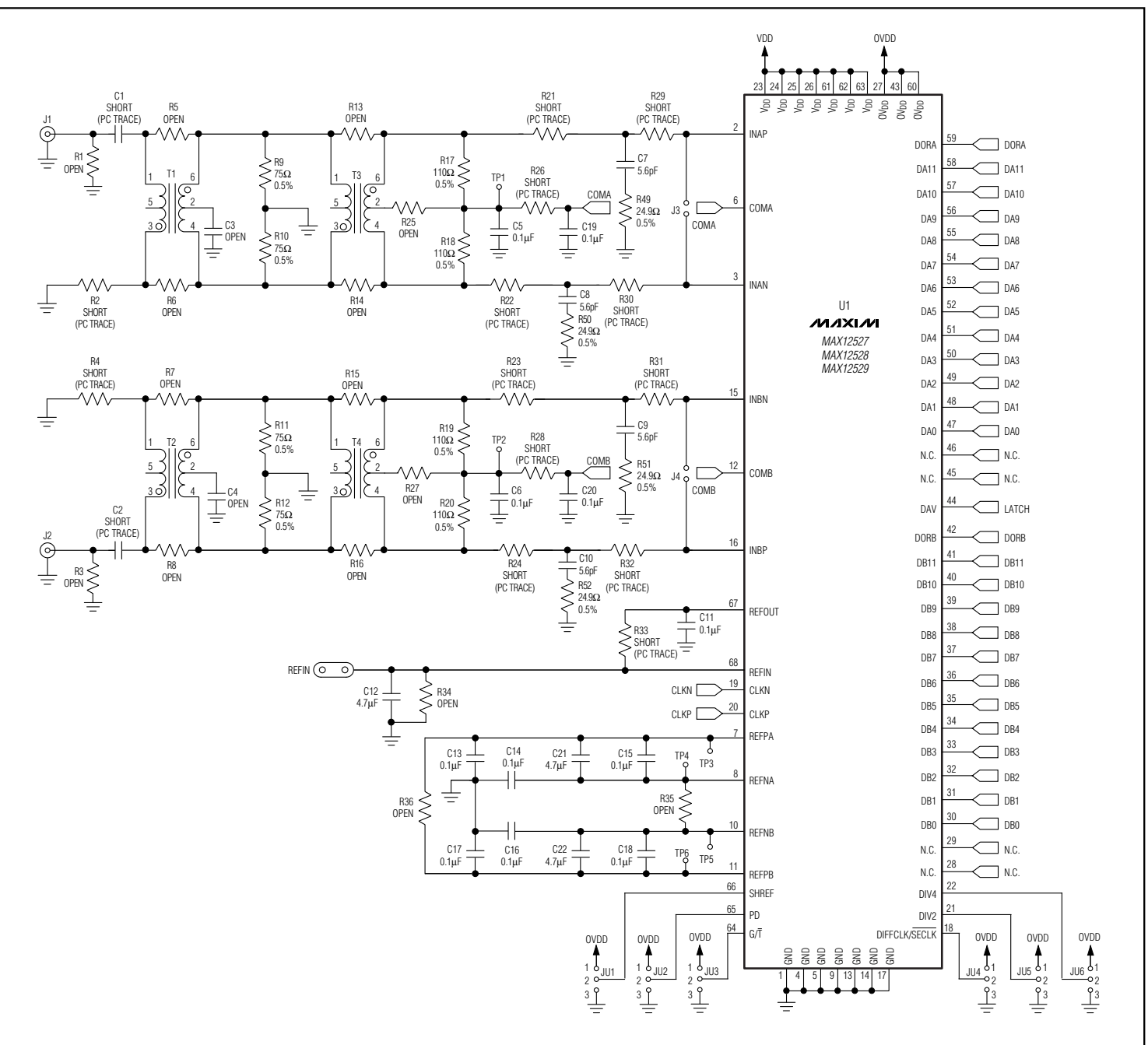
Figure 4. MAX12527/MAX12528/MAX12529 EV Kit Schematic (Sheet 1 of 4)
