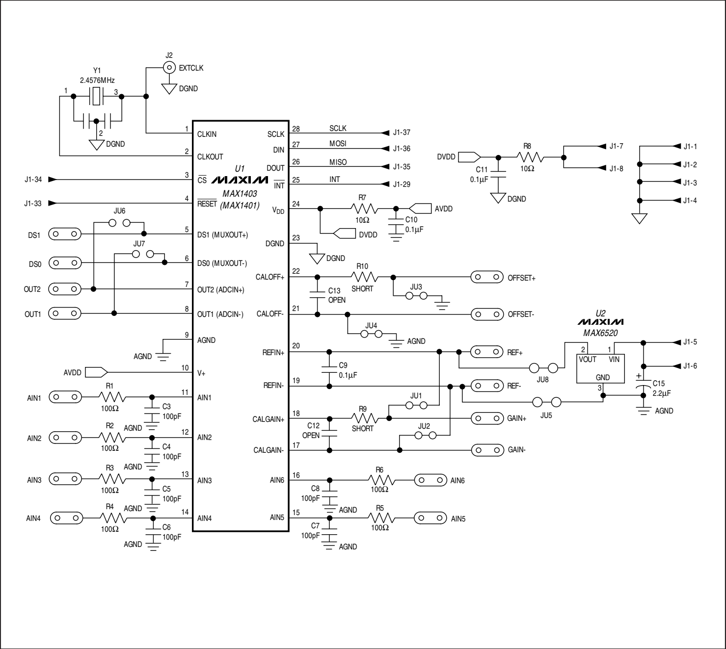
Figure 1. MAX1403 EV Kit Schematic
