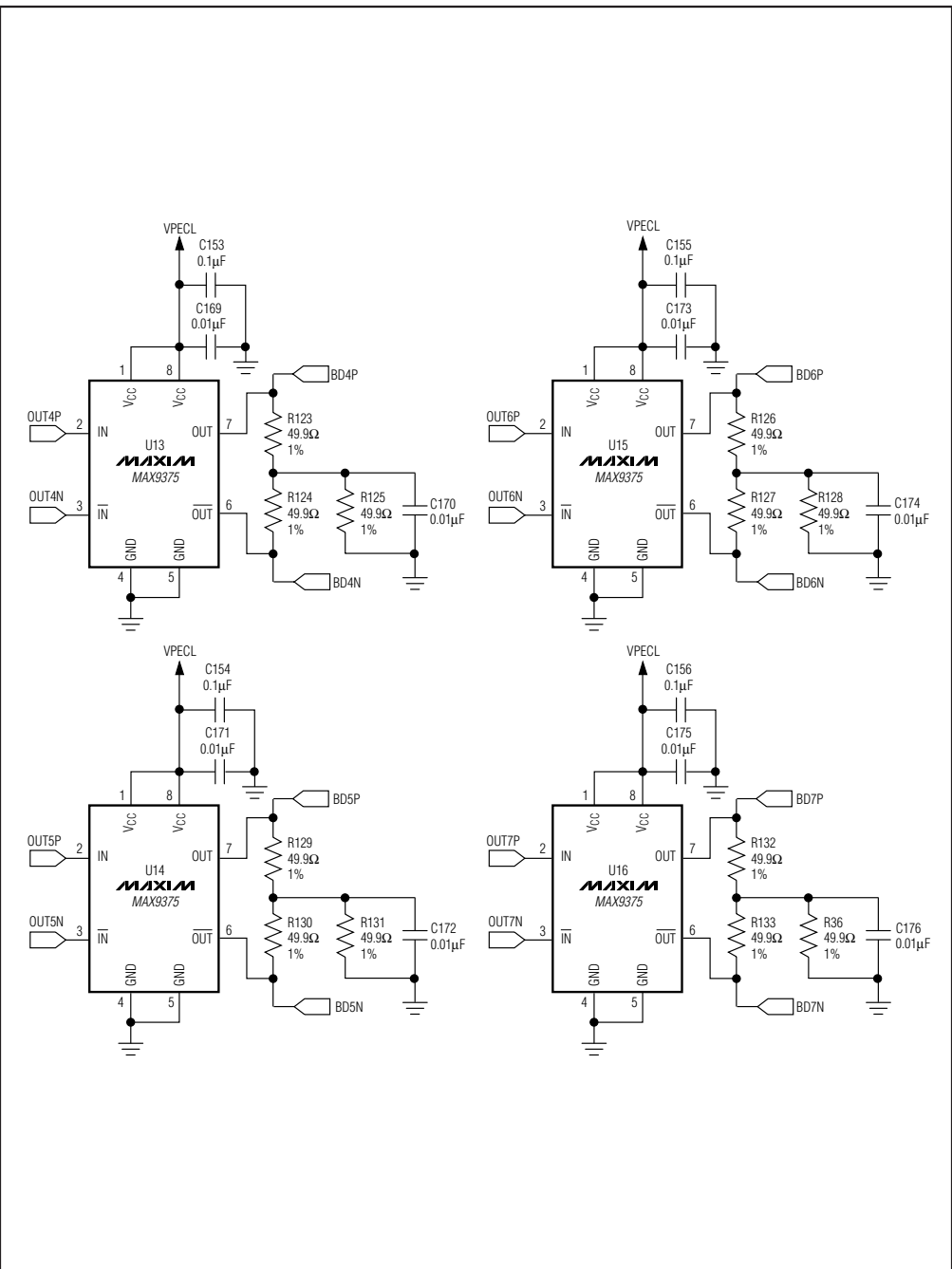
Figure 4. MAX1434/MAX1436/MAX1437/MAX1438 EV Kit Schematic—LVPECL Level Translators (Sheet 4 of 6)
