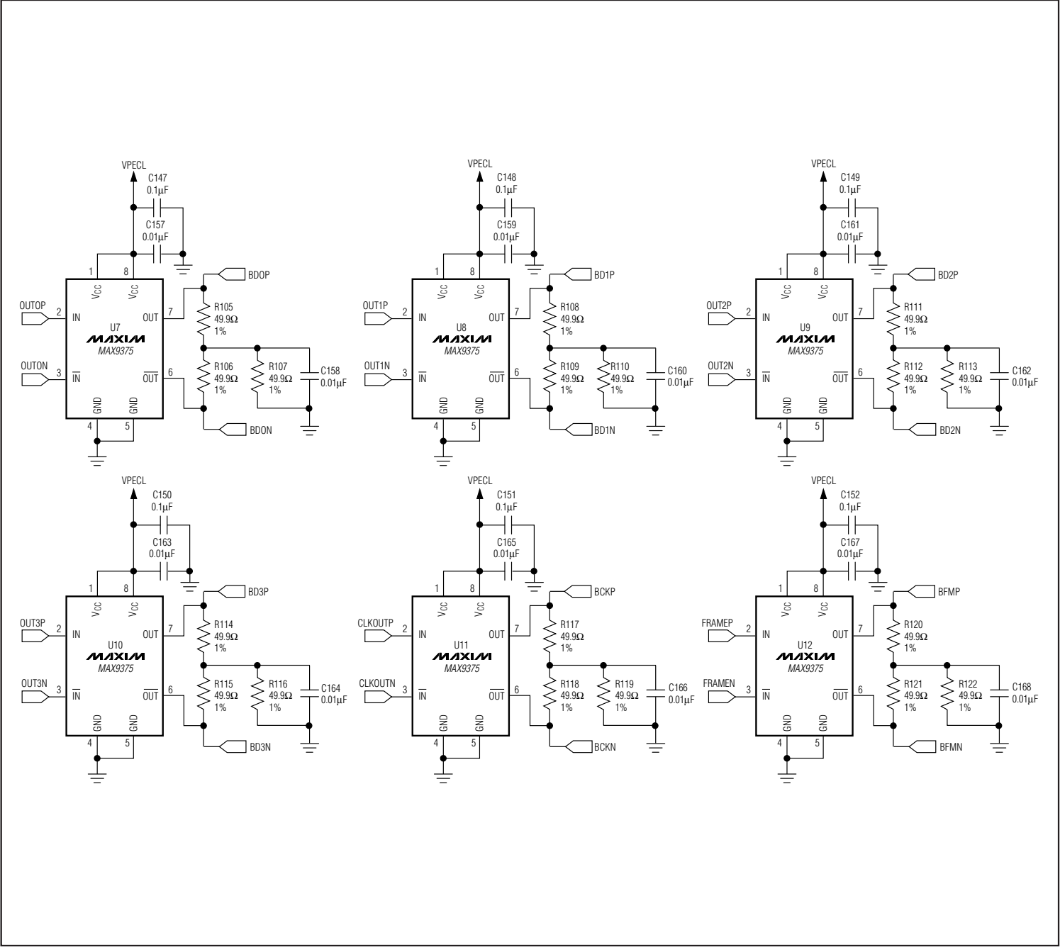
Figure 3. MAX1434/MAX1436/MAX1437/MAX1438 EV Kit Schematic—LVPECL Level Translators (Sheet 3 of 6)
