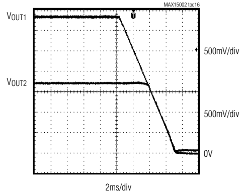
COINCIDENT SHUTDOWN
