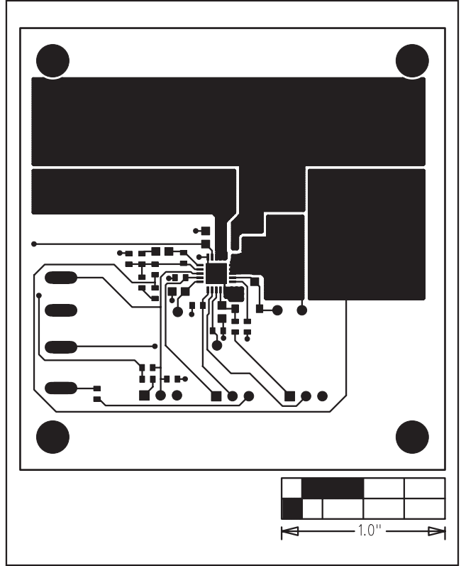
Figure 3. MAX15020 EV Kit PCB Layout—Component Side
