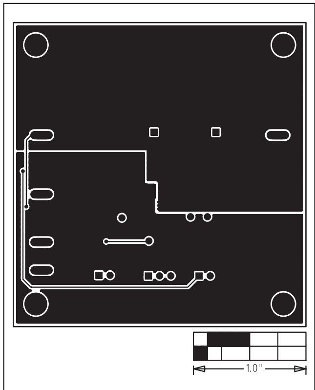
Figure 4. MAX15020 EV Kit PCB Layout—GND Layer 2
