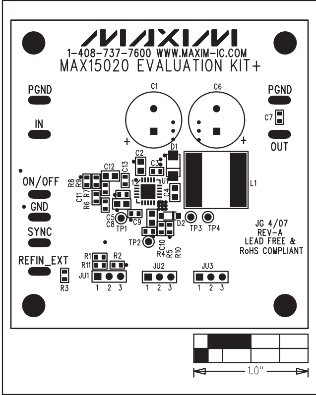
Figure 2. MAX15020 EV Kit Component Placement Guide—Component Side
