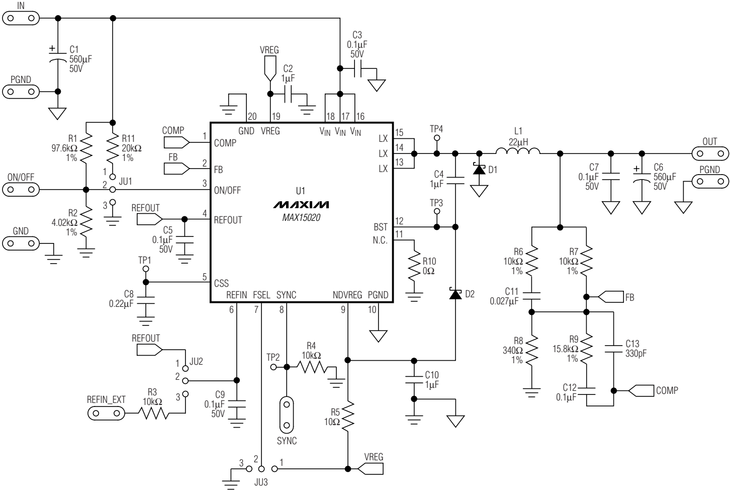
Figure 1. MAX15020 EV Kit Schematic
