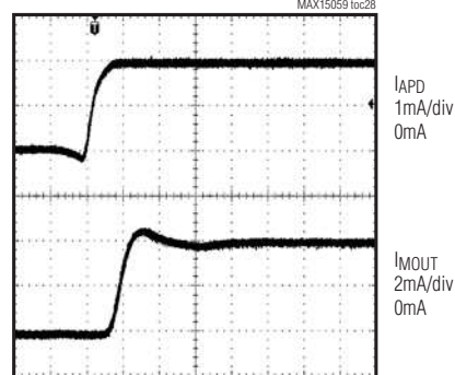
APD TRANSIENT RESPONSE (MAX15059A)
