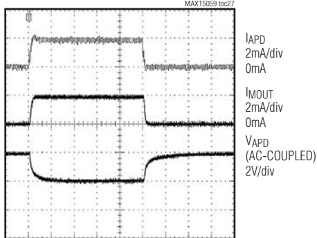
APD TRANSIENT RESPONSE (MAX15059A)
