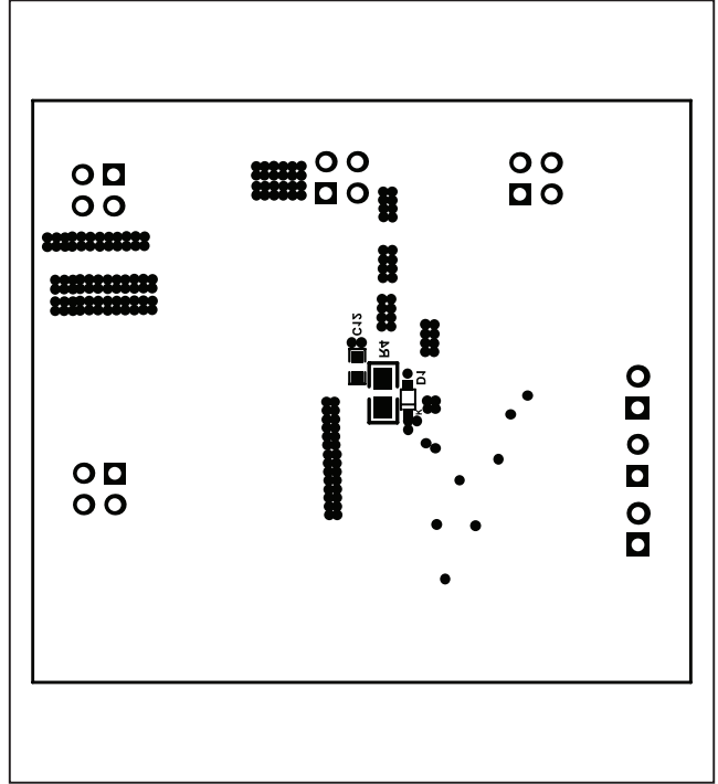
Figure 7. MAX15066 EV Kit Component Placement Guide—Solder Side
