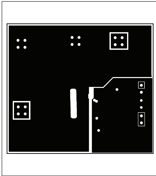
Figure 5. MAX15066 EV Kit PCB Layout—Inner Layer 3
