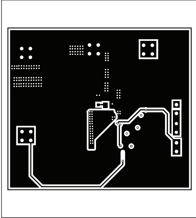
Figure 6. MAX15066 EV Kit PCB Layout—Solder Side
