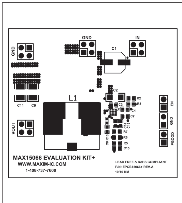
Figure 2. MAX15066 EV Kit Component Placement Guide—Component Side
