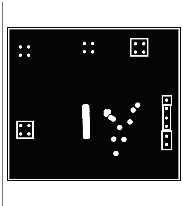
Figure 4. MAX15066 EV Kit PCB Layout—Inner Layer 2
