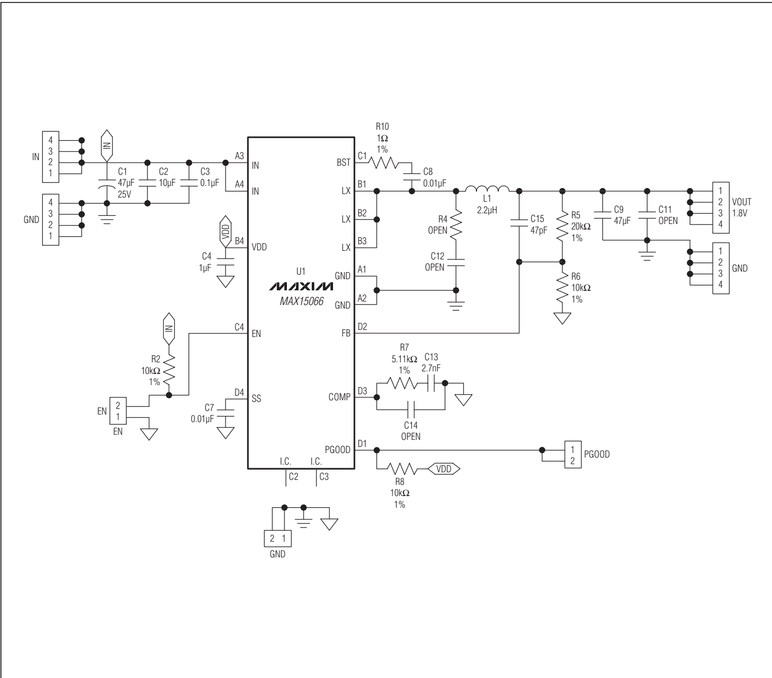
Figure 1. MAX15066 EV Kit Schematic
