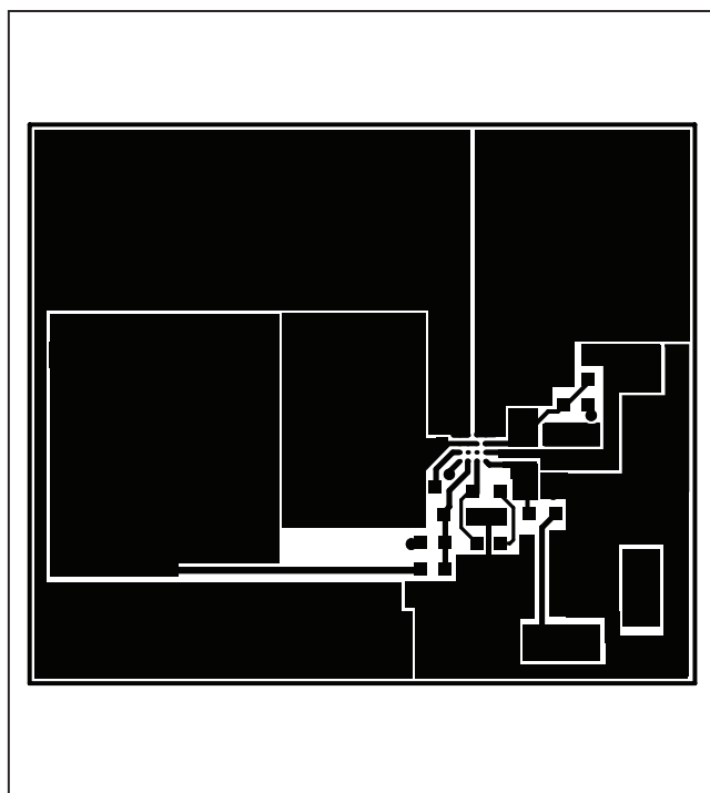
Figure 3. MAX15066 EV Kit PCB Layout—Component Side
