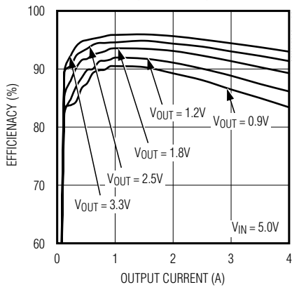
EFFICIENCY (5V) vs. OUTPUT CURRENT (MAX15166)
