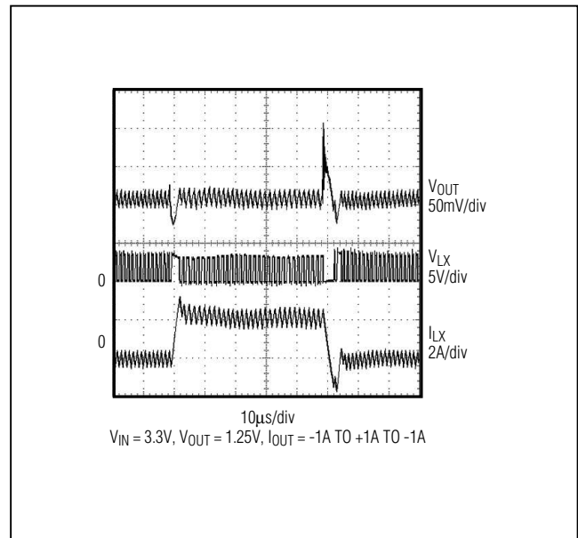
Figure 8. Source/Sink Waveforms
