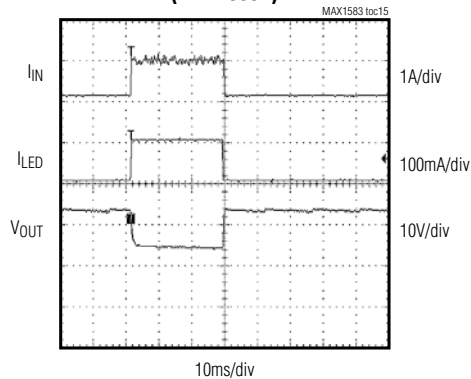
STROBE-PULSE WAVEFORMS (MAX1583X)
