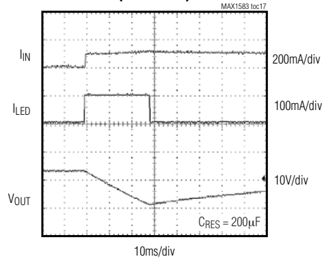
STROBE-PULSE WAVEFORMS (MAX1583Z)
