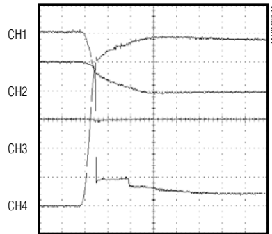
CURRENT-LIMIT RESPONSE
