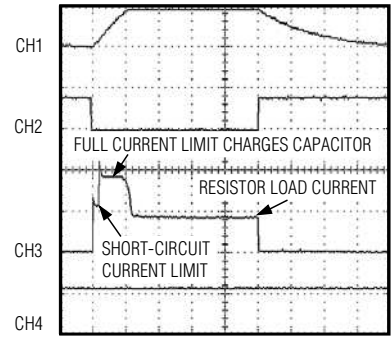
START-UP TIME (TYPICAL USB APPLICATION)
