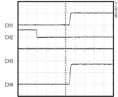
SWITCH TURN-ON TIME
