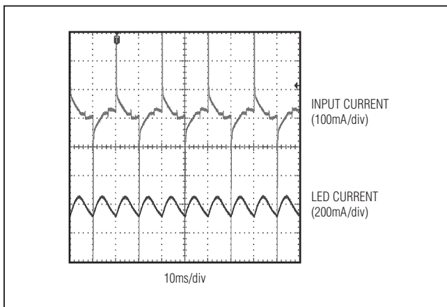
Figure 8. Dimmer at 50% Dimming Using Busch 2250
