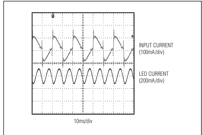
Figure 10. Dimmer at 100% Dimming Using Busch 6519
