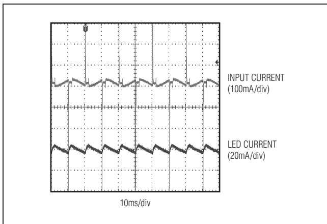
Figure 9. Dimmer at Very Low Dimming Using Busch 2250
