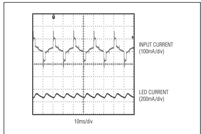
Figure 12. Dimmer at Very Low Dimming Using Busch 6519
