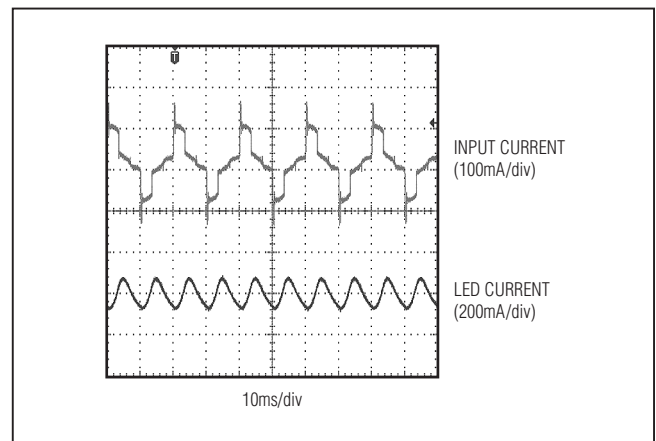
Figure 11. Dimmer at 50% Dimming Using Busch 6519
