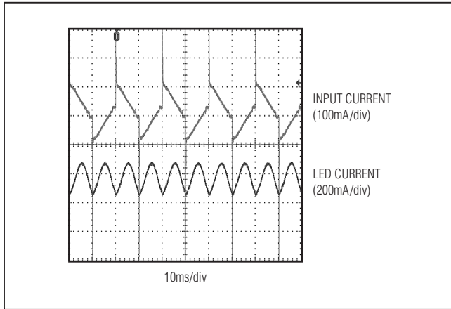
Figure 7. Dimmer At 100% Dimming Using Busch 2250
