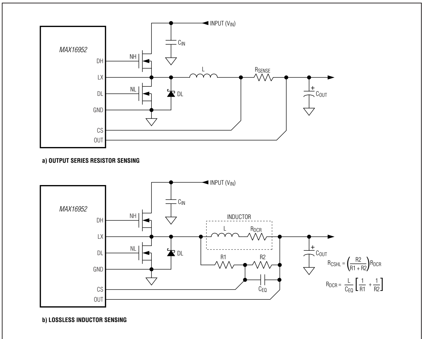
Figure 4. Current-Sense Configurations
