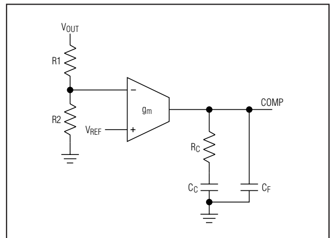
Figure 5. Compensation Network
