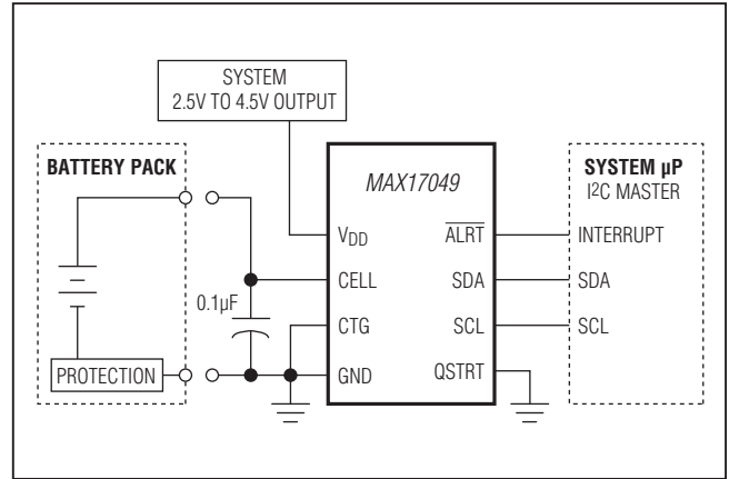
Figure 15. MAX17049 Application Circuit (2S Cell Pack)
