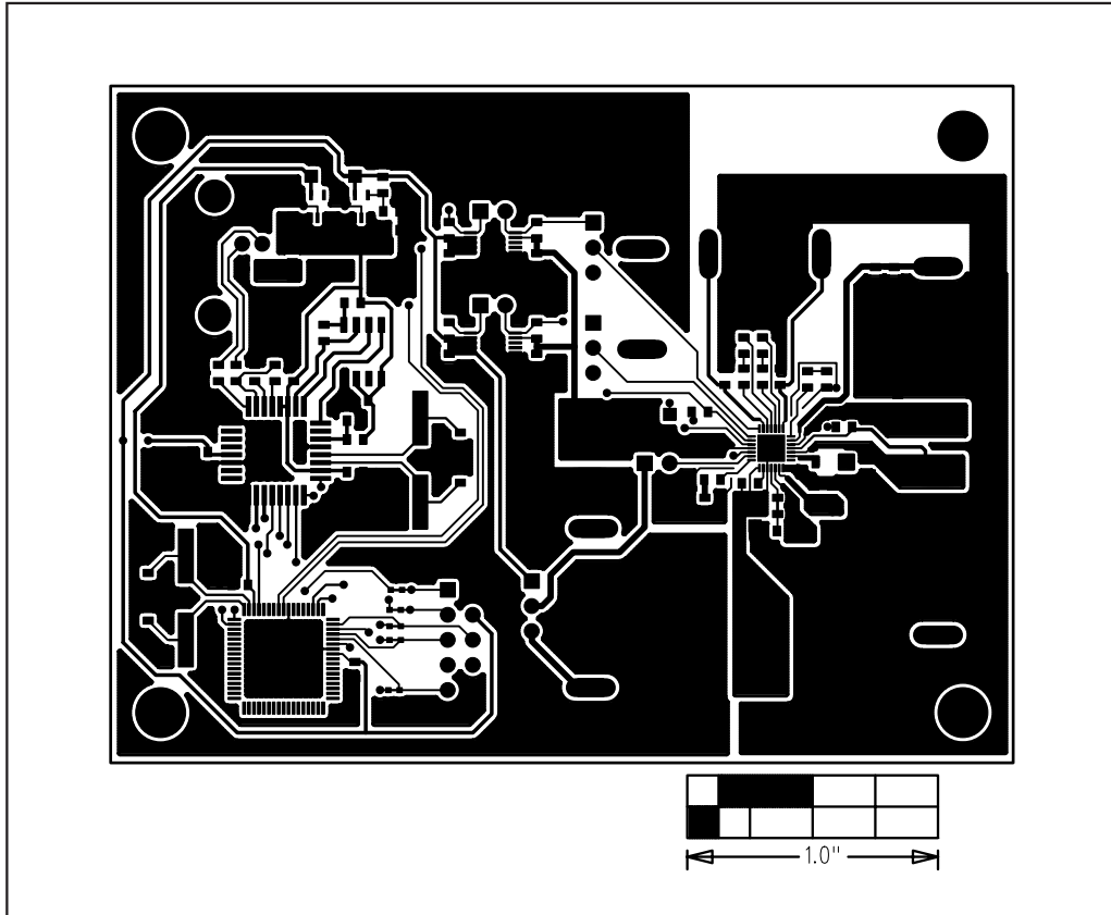
Figure 6. MAX17065 EV Kit PCB Layout—Component Side
