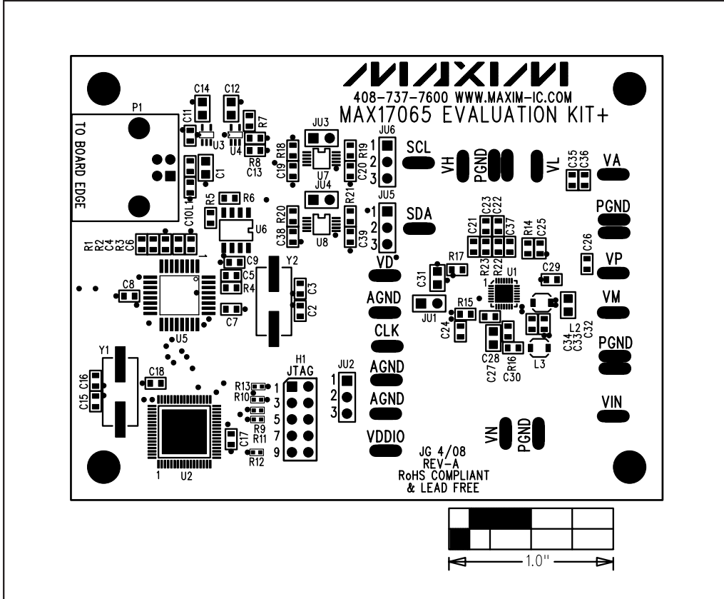
Figure 5. MAX17065 EV Kit Component Placement Guide—Component Side
