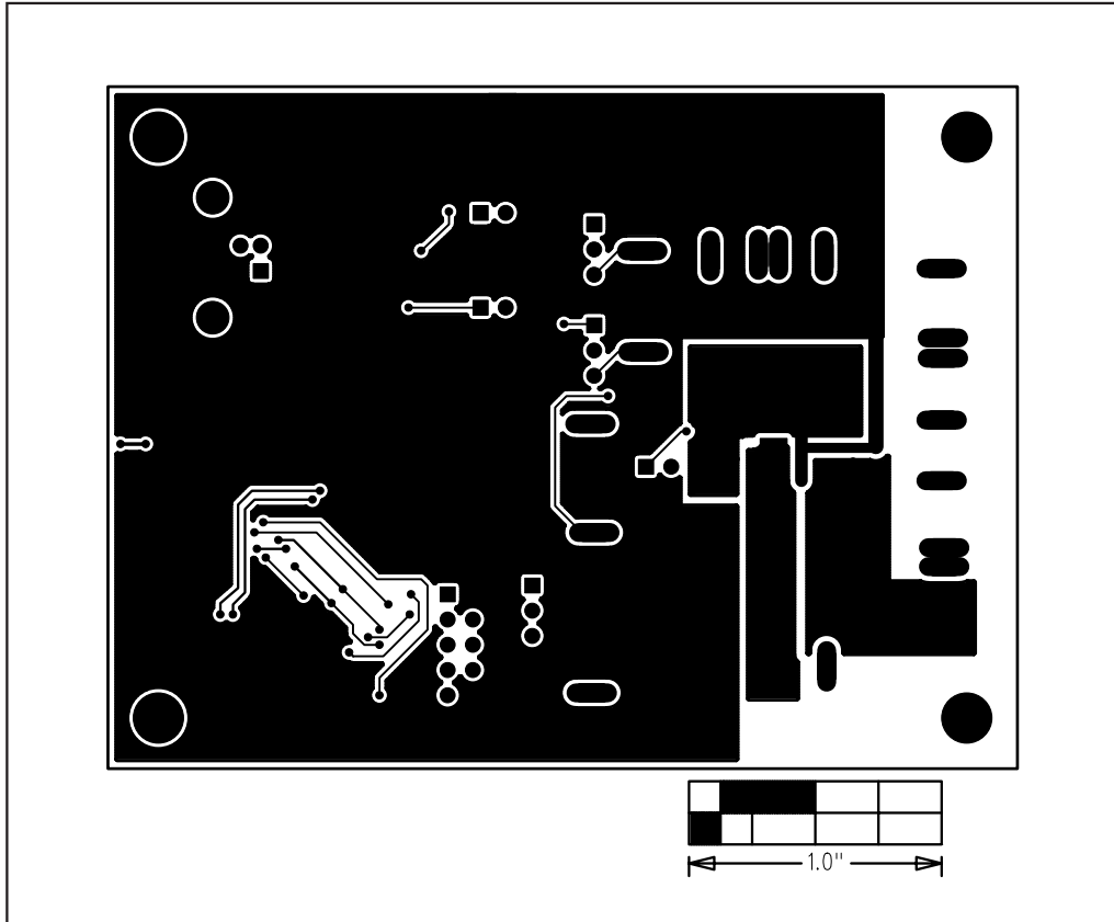
Figure 7. MAX17065 EV Kit PCB Layout—Solder Side
