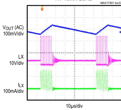
SWITCHING WAVEFORMS OF MAX17501A AT 15mA LOAD
