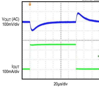
LOAD TRANSIENT RESPONSE OF MAX17501F (LOAD CURRENT STEPPED FROM NO-LOAD TO 250mA)
