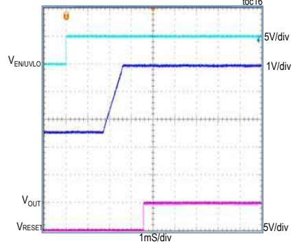
MAX17574, SOFT-START WITH 2.5V PREBIAS, 5V OUTPUT, PWM MODE, FIGURE 3 CIRCUIT
