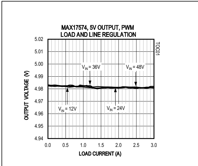
Figure 1. MAX17574 5V Output Load and Line Regulation (PWM Mode)
