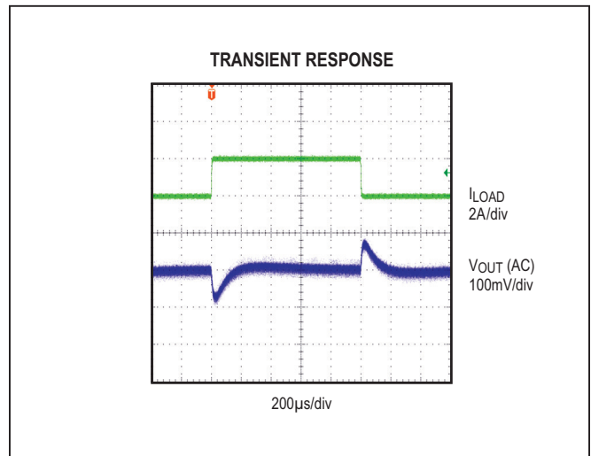
Figure 3. Transient Response
