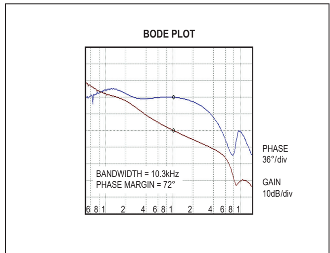
Figure 4. Bode Plot
