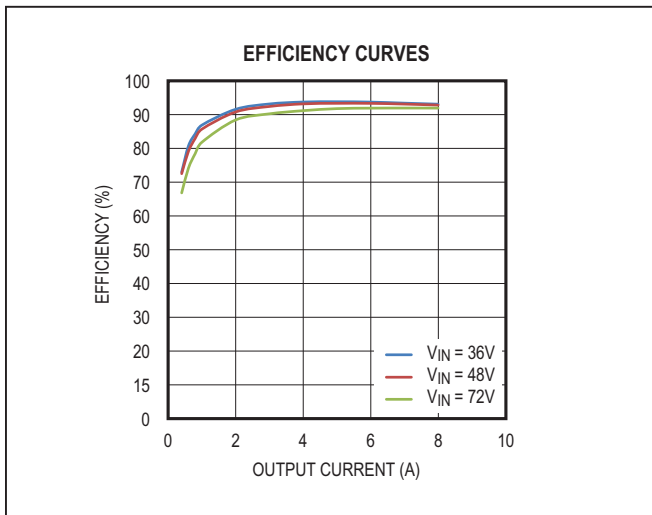
Figure 1. Efficiency Curves
