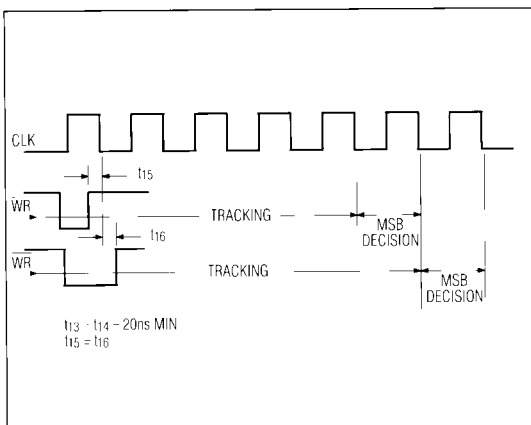
Figure 7. Width of Tracking Interval as a Function of \overline{\text{WR}} Rising Edge Timing with Respect to CLK Falling Edge
