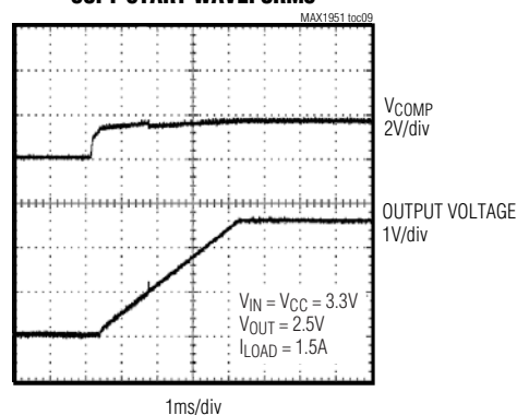
SOFT-START WAVEFORMS
