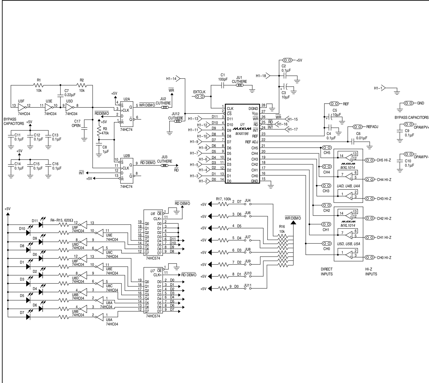
Figure 2. MAX196 EV Kit Schematic
