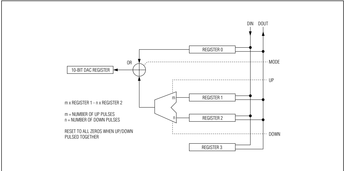
Figure 1. Register Configuration Diagram
