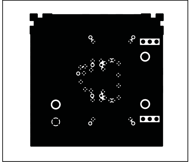
Figure 9. MAX2021 EV Kit PCB Layout—Bottom Layer (Metal)
