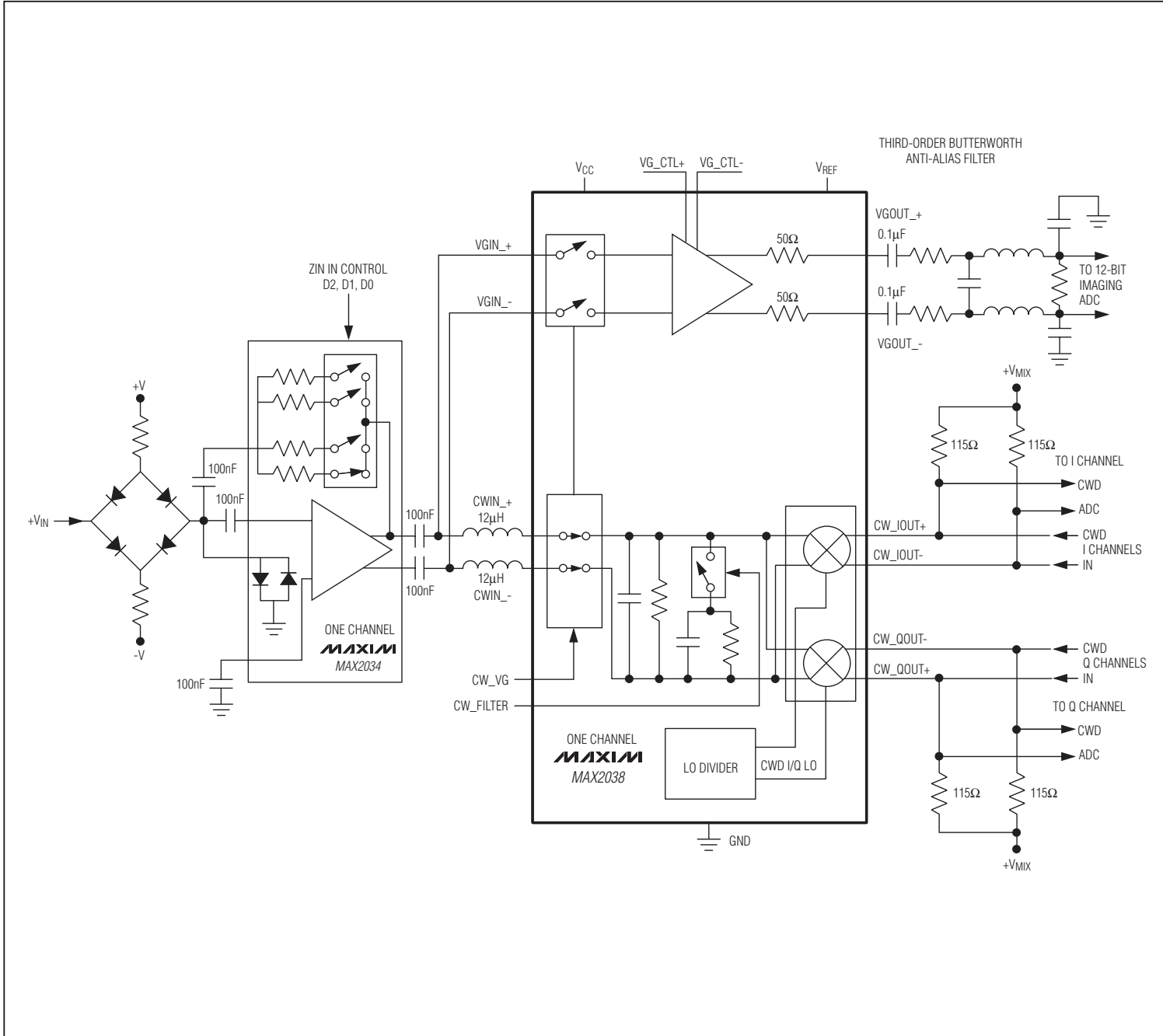
Figure 7. Typical Per-Channel Ultrasound Imaging Application
