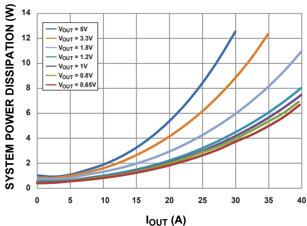
SYSTEM POWER DISSIPATION
