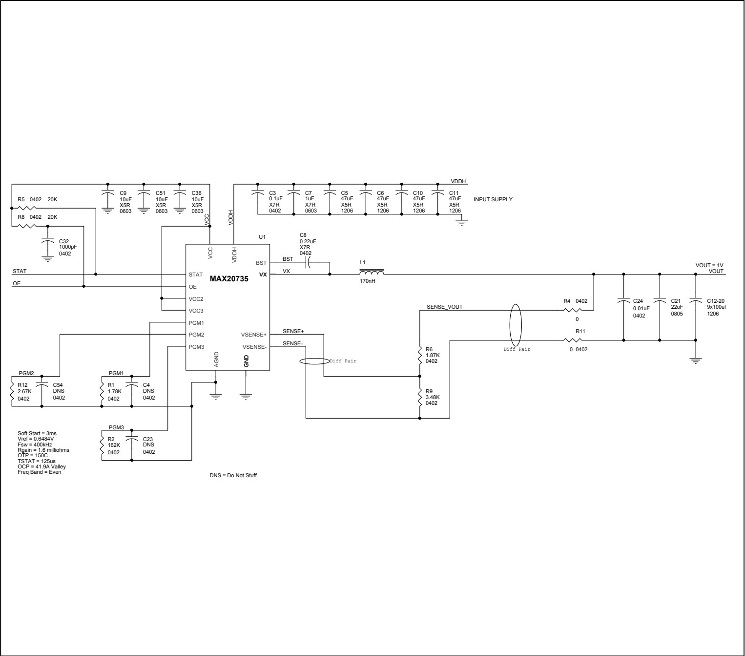
Figure 6. Reference Schematic (VDDH = 4.5V to 16V, VOUT = 1V)
