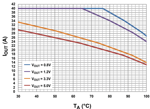
SAFE OPERATING AREA (SOA)
