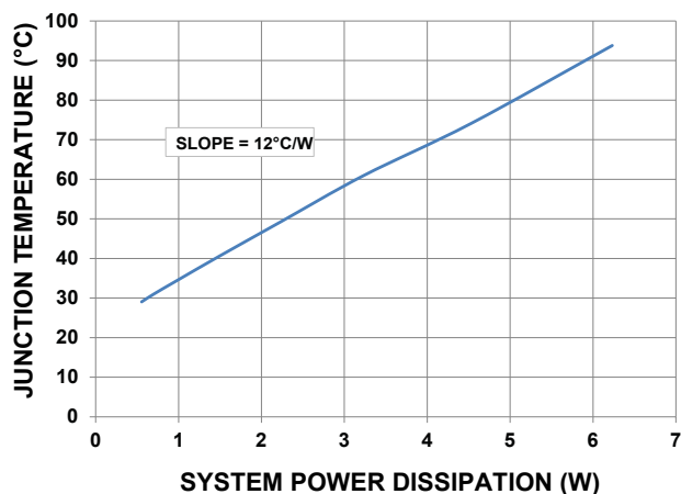
JUNCTION TEMPERATURE vs. SYSTEM POWER DISSIPATION
