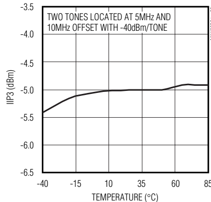
IIP3 vs. TEMPERATURE
