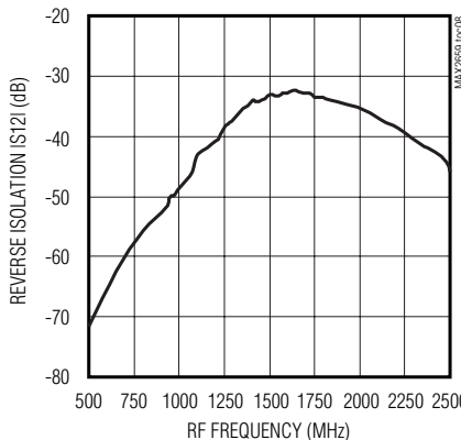
REVERSE ISOLATION vs. RF FREQUENCY
