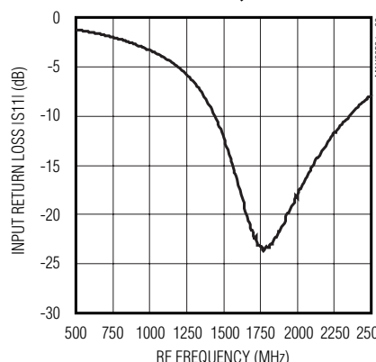
INPUT RETURN LOSS vs. RF FREQUENCY
