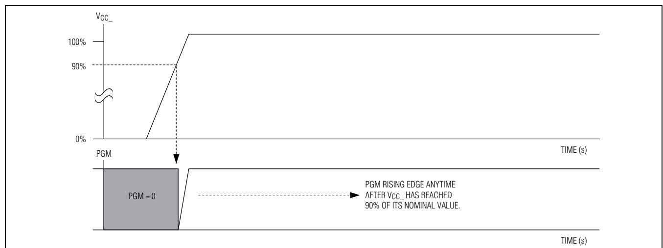
Figure 4. V_{CC\_} Power-On Reset
