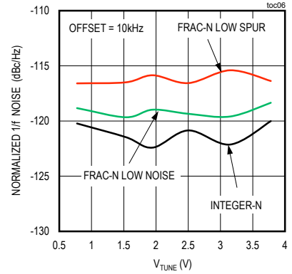
NORMALIZED 1/f NOISE vs. TUNE VOLTAGE
