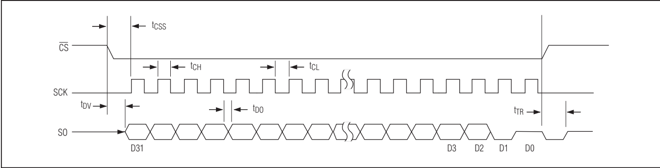
Figure 2. Serial-Interface Timing
