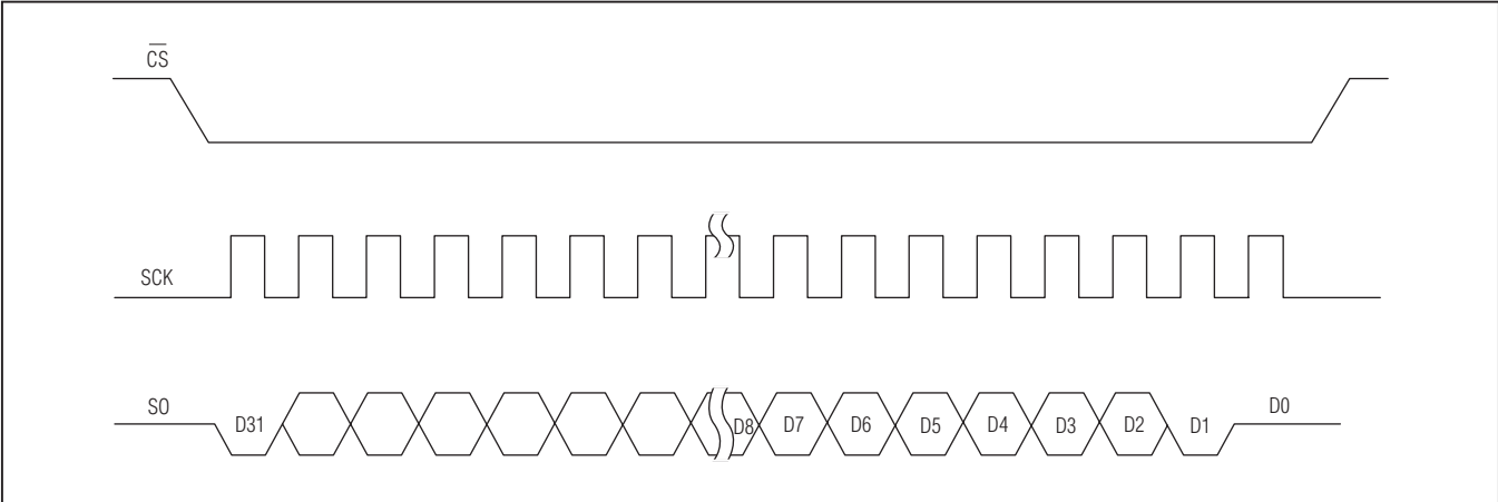
Figure 1. Serial-Interface Protocol
