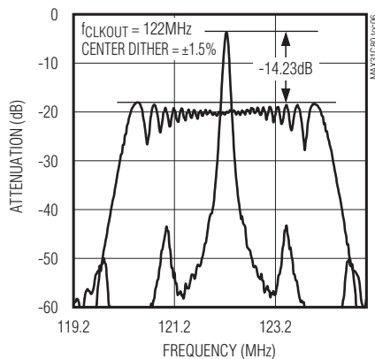
FREQUENCY SPECTRUM AT 122MHz WITH CENTER SPREAD
