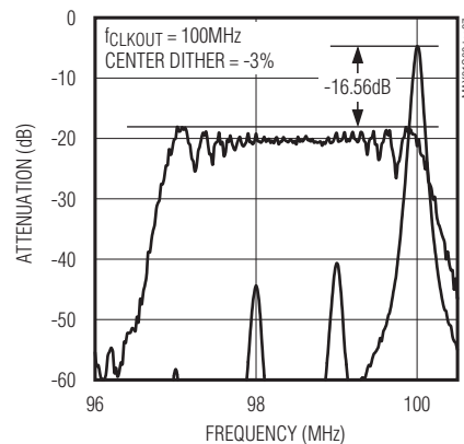
FREQUENCY SPECTRUM AT 100MHz WITH DOWN DITHER
