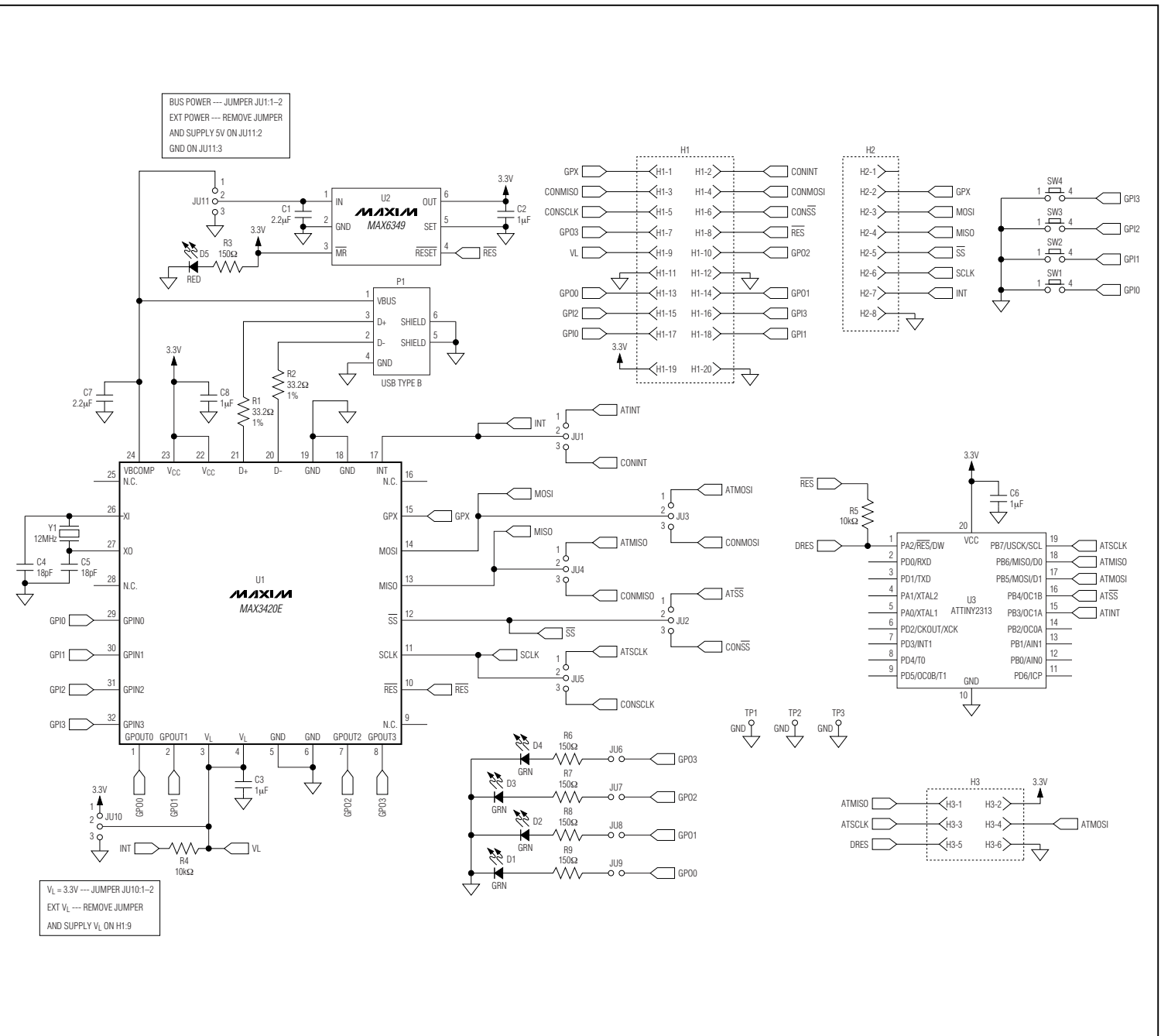
Figure 3. MAX3420E EV Kit-2 Schematic
