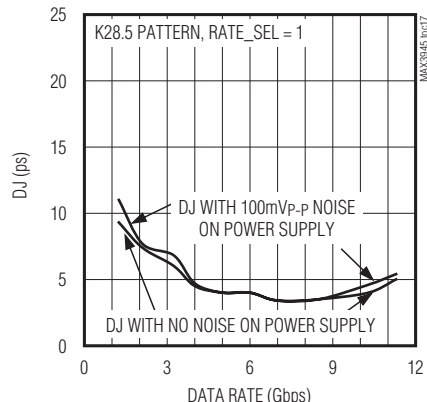
DETERMINISTIC JITTER vs. DATA RATE (INPUT = 100mVp-p)
