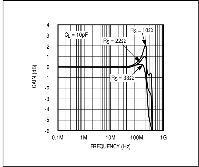
Figure 3b. MAX4102 Bandwidth vs. 10pF Capacitive Load and Isolation Resistor
