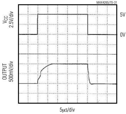
POWER-UP/POWER-DOWN RESPONSE
