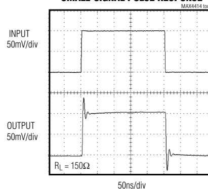
MAX4414/MAX4416/MAX4418 SMALL-SIGNAL PULSE RESPONSE
