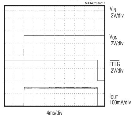
FFLG-BLANKING RESPONSE
