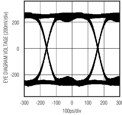
V_{IN} = 1600\text{mVp-p} , 3.0Gbps, PA = 0, PB = 0
