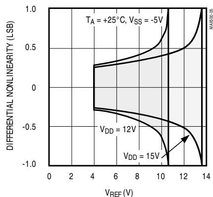
DIFFERENTIAL NONLINEARITY vs. REFERENCE VOLTAGE
