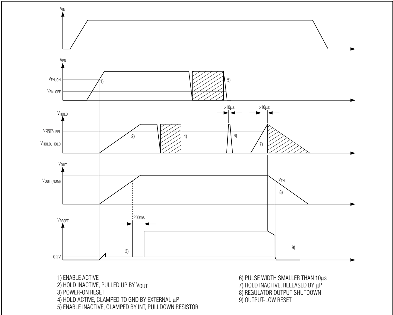
Figure 3. Enable and Hold Behavior
