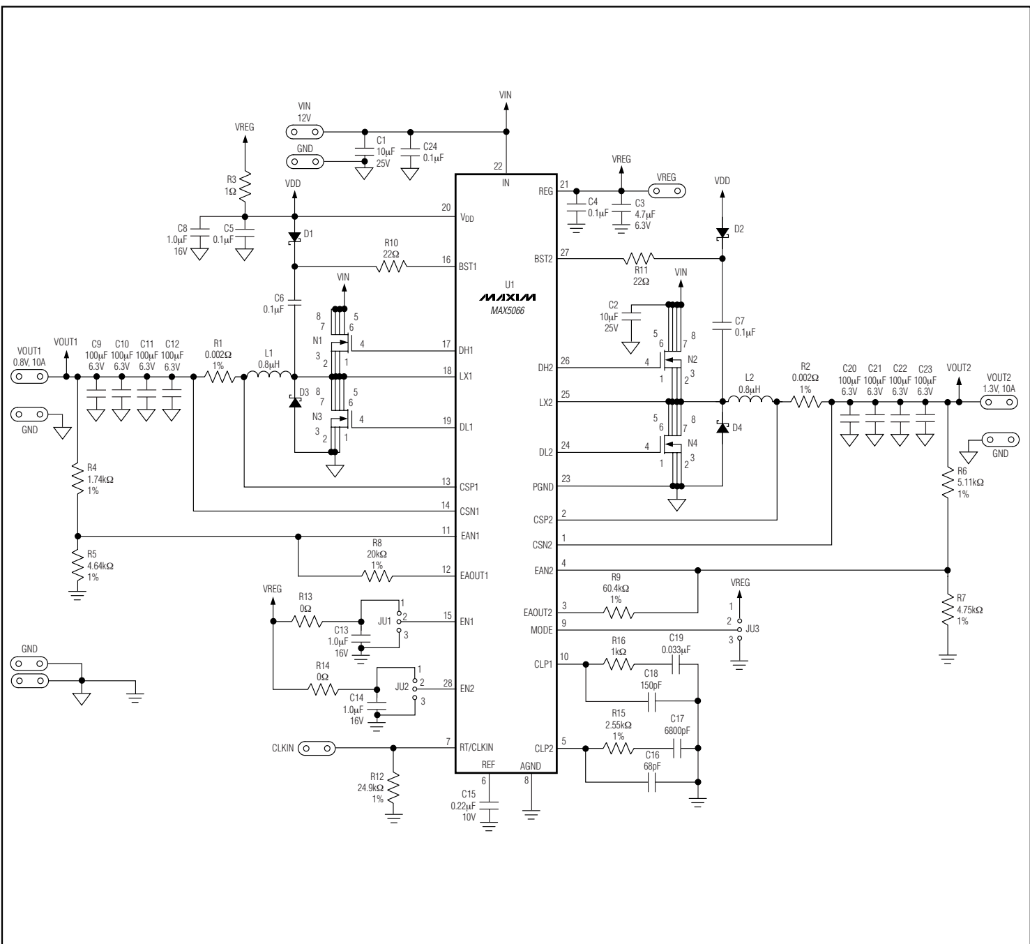
Figure 1. MAX5066 EV Kit Schematic
