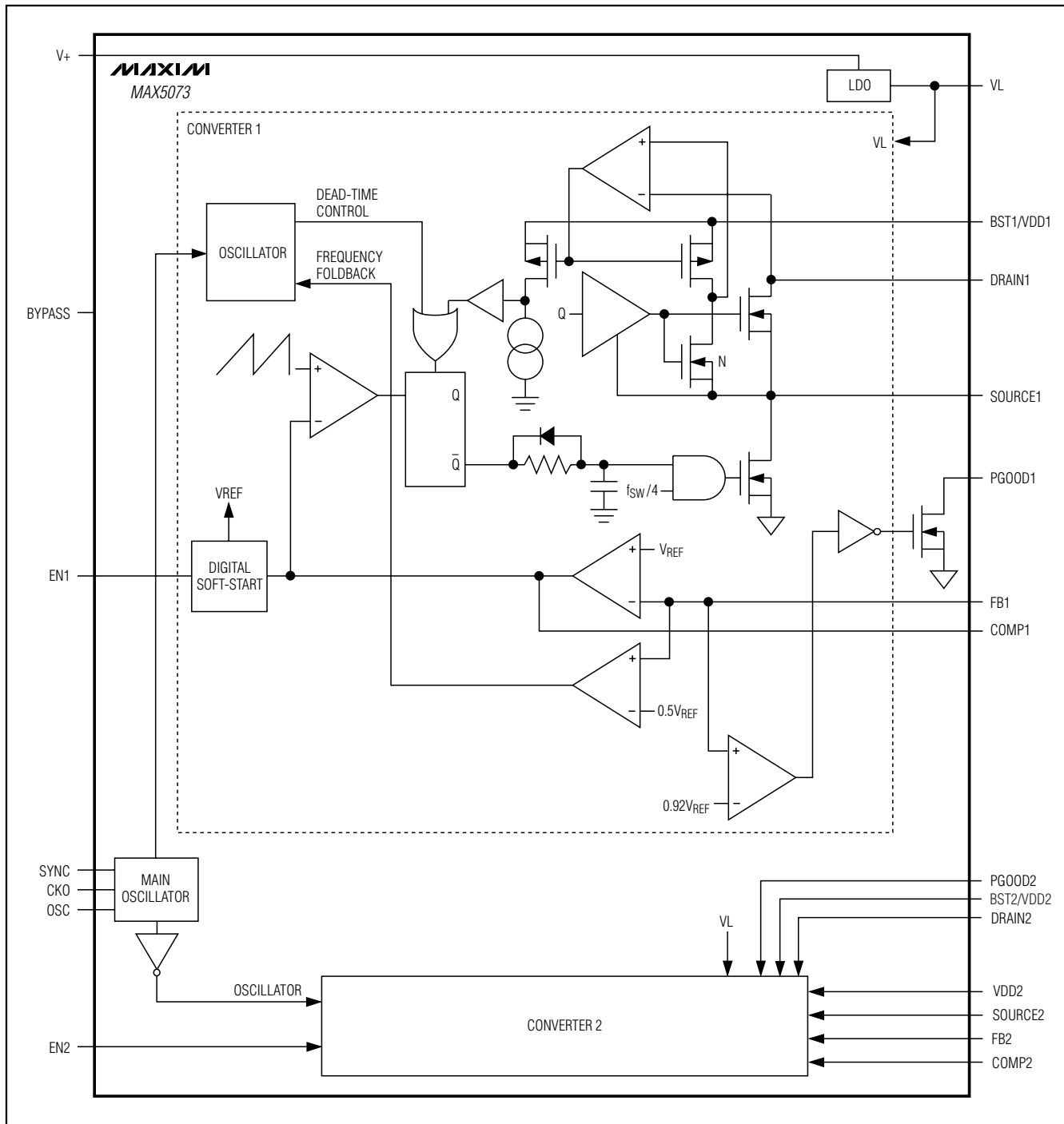
Figure 2. Functional Diagram
