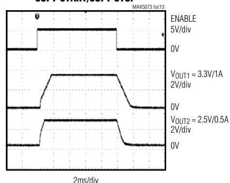
SOFT-START/SOFT-STOP
