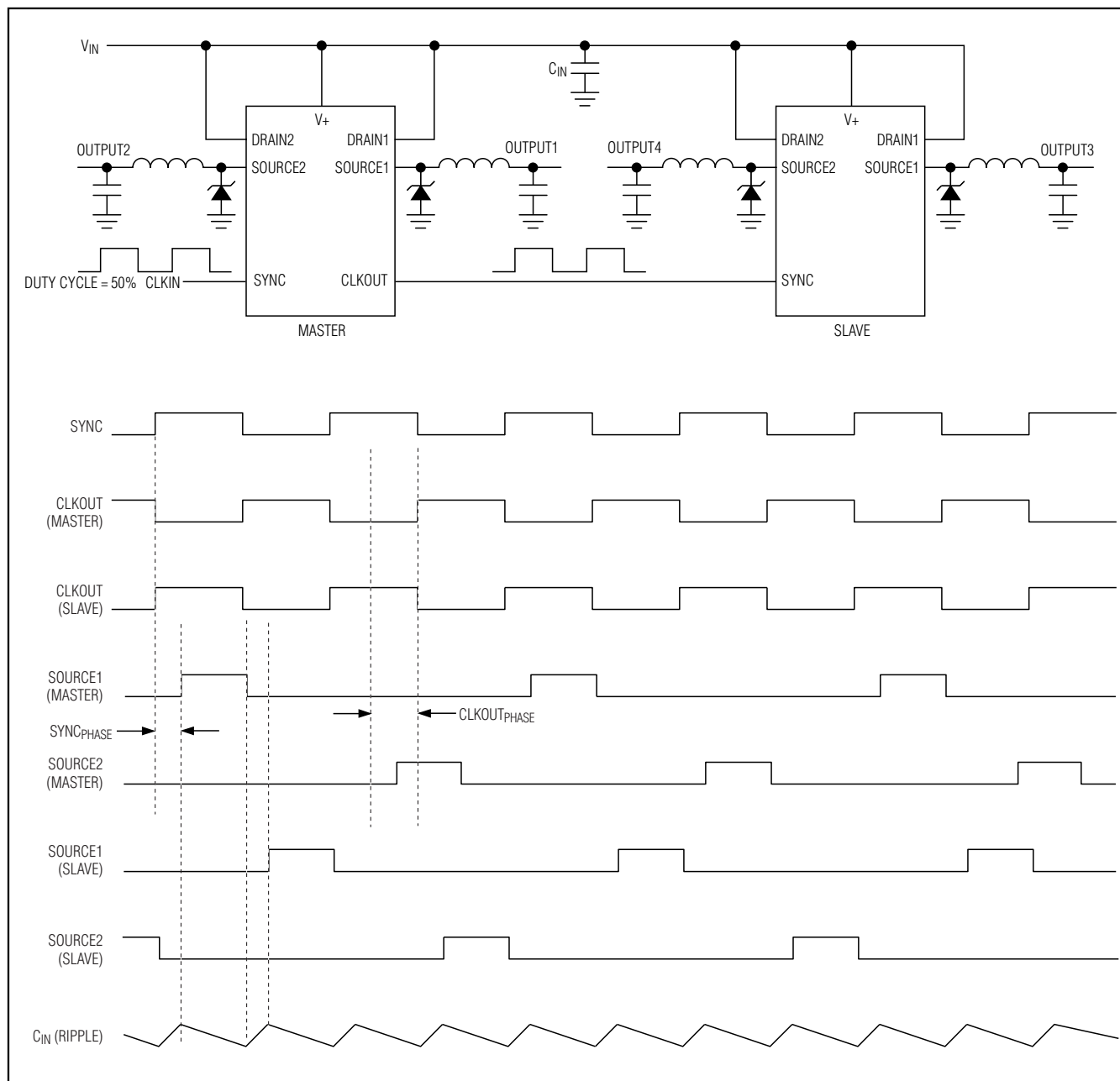
Figure 3. Synchronized Controllers
